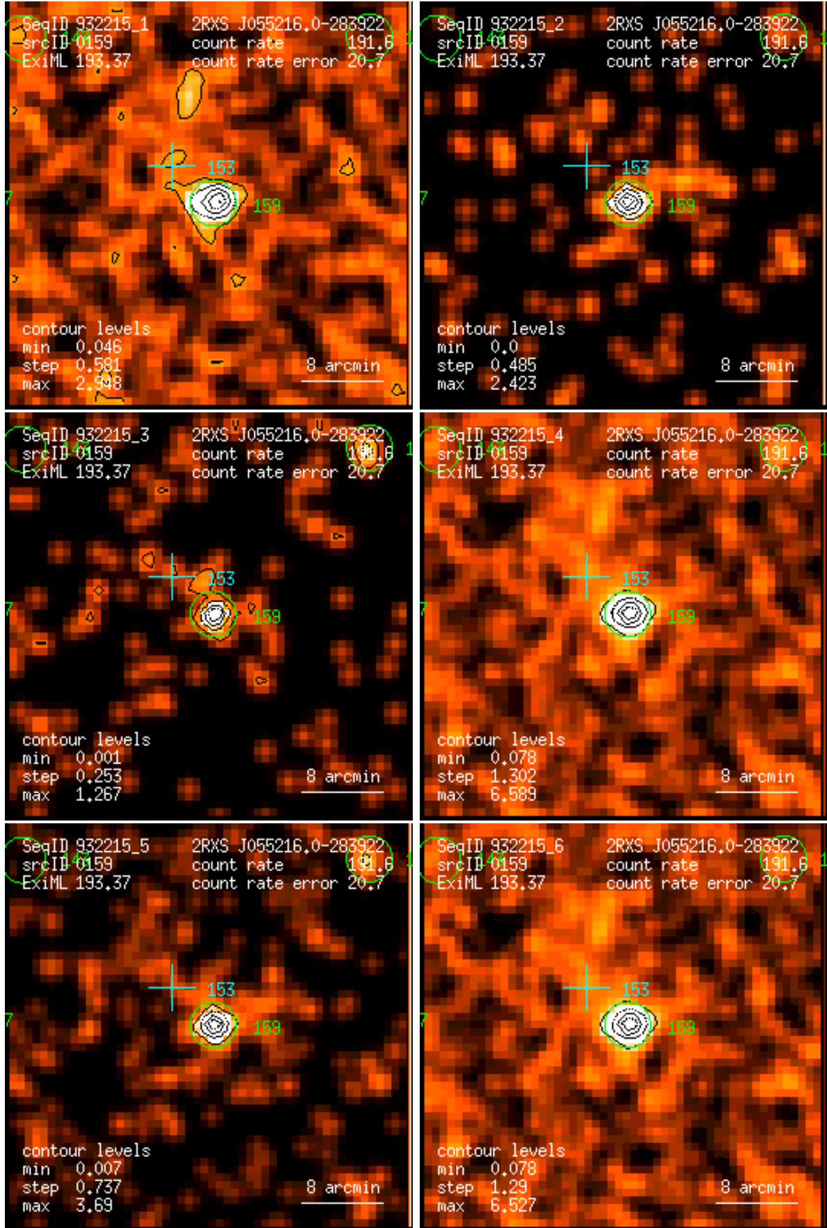
Figure 159: RASS 932215: detection 0159: band rate images, Gaussian filter: (1) PSPC channels 11 – 41, (2) 52 – 90, (3) 91 – 201, (4) 11 – 235, (5) 52 – 201, (6) 11 – 201. Broad band rates in counts/ks. Band rate contour levels in counts/ks/arcmin 2 .
