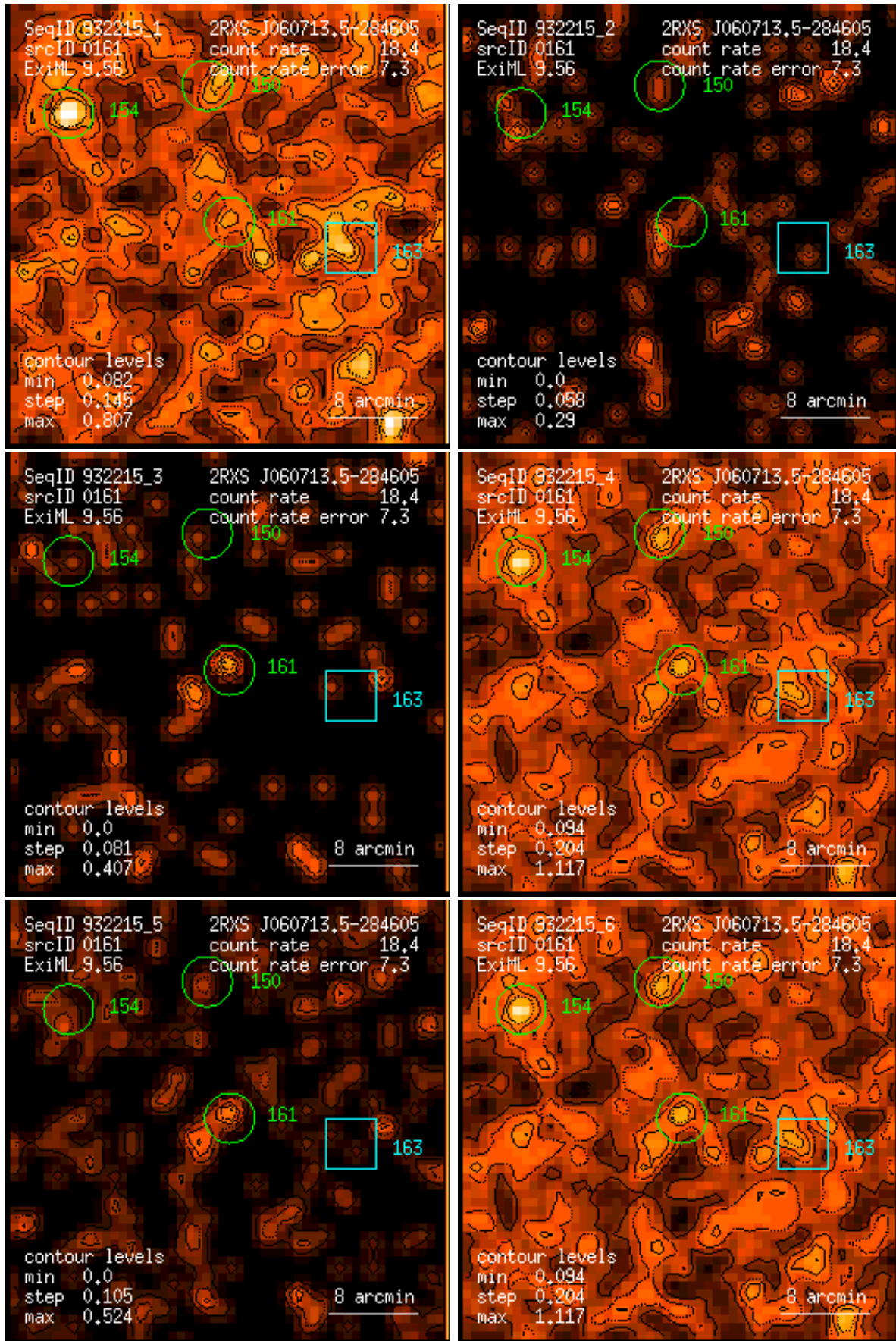
Figure 161: RASS 932215: detection 0161: band rate images, Gaussian filter: (1) PSPC channels 11 – 41, (2) 52 – 90, (3) 91 – 201, (4) 11 – 235, (5) 52 – 201, (6) 11 – 201. Broad band rates in counts/ks. Band rate contour levels in counts/ks/arcmin 2 .
