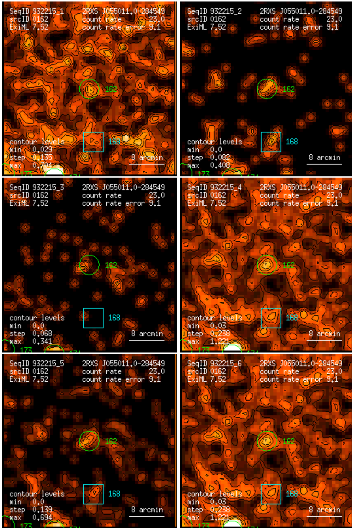
Figure 162: RASS 932215: detection 0162: band rate images, Gaussian filter: (1) PSPC channels 11 – 41, (2) 52 – 90, (3) 91 – 201, (4) 11 – 235, (5) 52 – 201, (6) 11 – 201. Broad band rates in counts/ks. Band rate contour levels in counts/ks/arcmin 2 .
