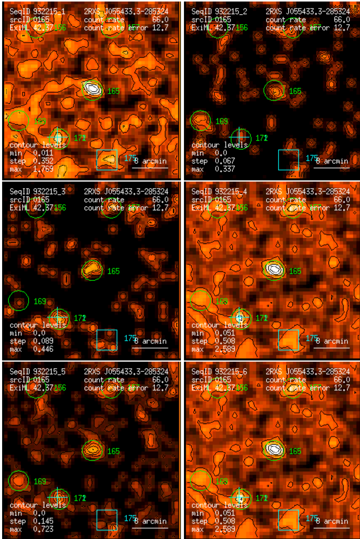
Figure 165: RASS 932215: detection 0165: band rate images, Gaussian filter: (1) PSPC channels 11 – 41, (2) 52 – 90, (3) 91 – 201, (4) 11 – 235, (5) 52 – 201, (6) 11 – 201. Broad band rates in counts/ks. Band rate contour levels in counts/ks/arcmin 2 .
