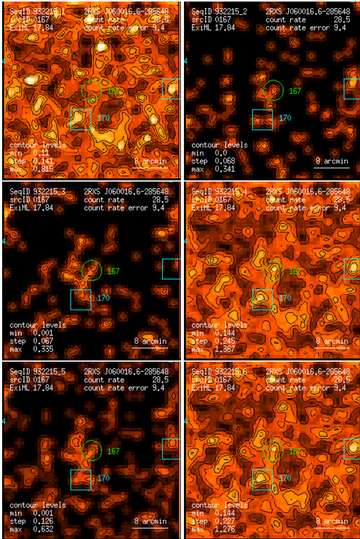
Figure 167: RASS 932215: detection 0167: band rate images, Gaussian filter: (1) PSPC channels 11 – 41, (2) 52 – 90, (3) 91 – 201, (4) 11 – 235, (5) 52 – 201, (6) 11 – 201. Broad band rates in counts/ks. Band rate contour levels in counts/ks/arcmin 2 .
