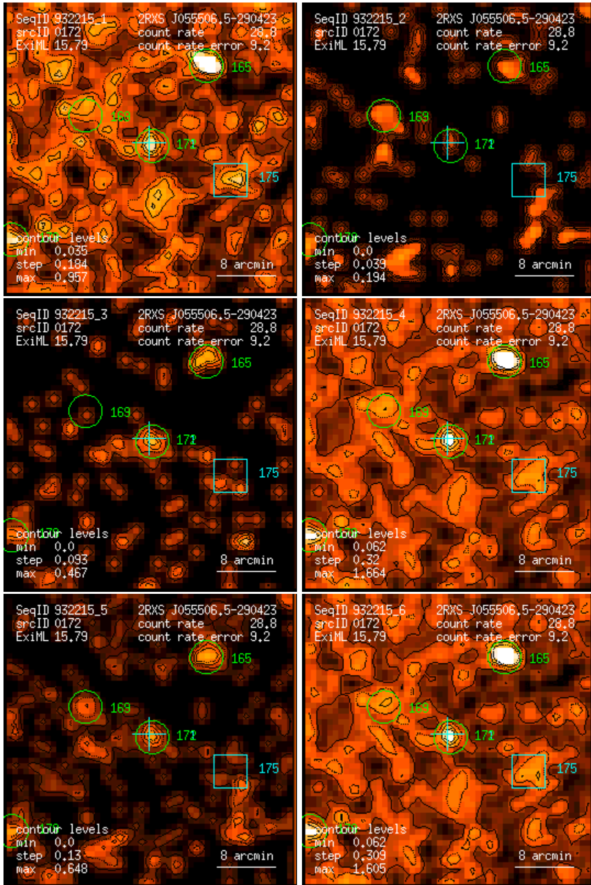
Figure 172: RASS 932215: detection 0172: band rate images, Gaussian filter: (1) PSPC channels 11 – 41, (2) 52 – 90, (3) 91 – 201, (4) 11 – 235, (5) 52 – 201, (6) 11 – 201. Broad band rates in counts/ks. Band rate contour levels in counts/ks/arcmin 2 .
