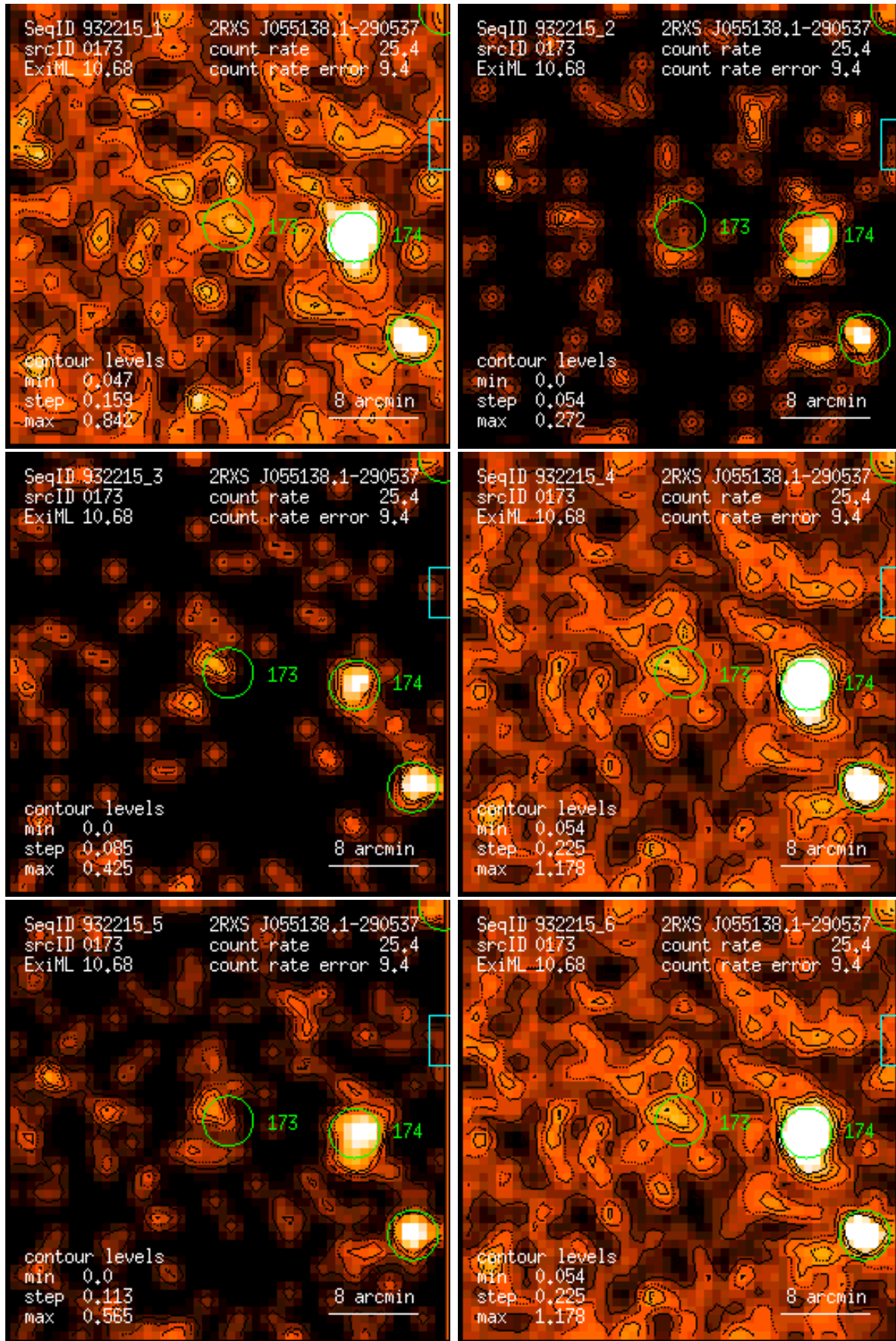
Figure 173: RASS 932215: detection 0173: band rate images, Gaussian filter: (1) PSPC channels 11 – 41, (2) 52 – 90, (3) 91 – 201, (4) 11 – 235, (5) 52 – 201, (6) 11 – 201. Broad band rates in counts/ks. Band rate contour levels in counts/ks/arcmin 2 .
