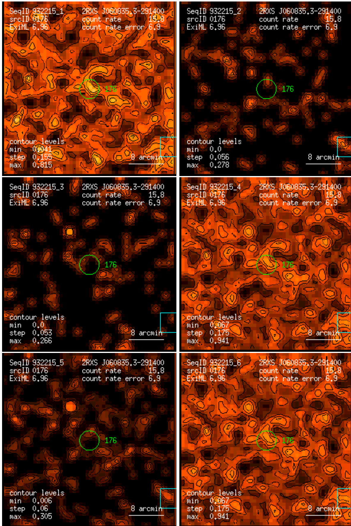
Figure 176: RASS 932215: detection 0176: band rate images, Gaussian filter: (1) PSPC channels 11 – 41, (2) 52 – 90, (3) 91 – 201, (4) 11 – 235, (5) 52 – 201, (6) 11 – 201. Broad band rates in counts/ks. Band rate contour levels in counts/ks/arcmin 2 .
