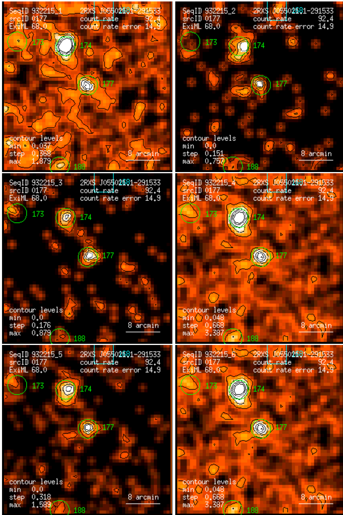
Figure 177: RASS 932215: detection 0177: band rate images, Gaussian filter: (1) PSPC channels 11 – 41, (2) 52 – 90, (3) 91 – 201, (4) 11 – 235, (5) 52 – 201, (6) 11 – 201. Broad band rates in counts/ks. Band rate contour levels in counts/ks/arcmin 2 .
