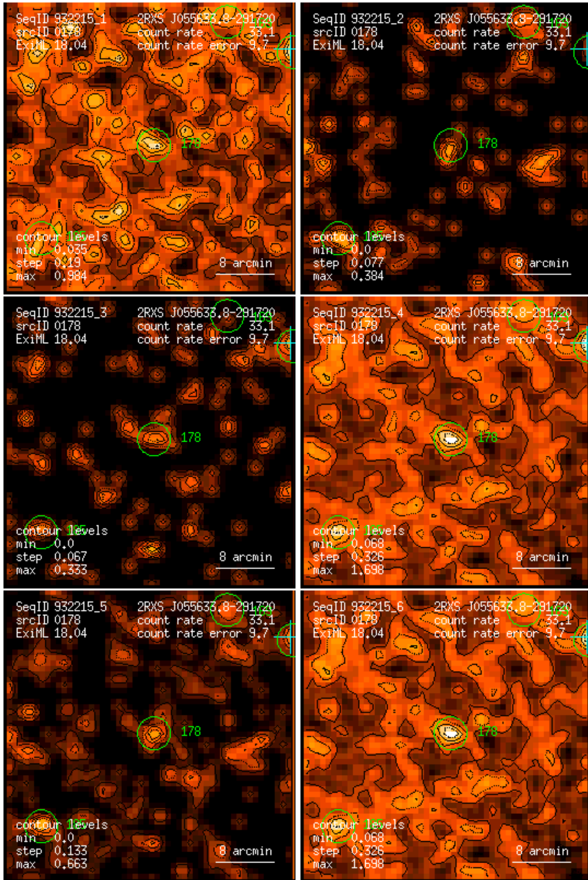
Figure 178: RASS 932215: detection 0178: band rate images, Gaussian filter: (1) PSPC channels 11 – 41, (2) 52 – 90, (3) 91 – 201, (4) 11 – 235, (5) 52 – 201, (6) 11 – 201. Broad band rates in counts/ks. Band rate contour levels in counts/ks/arcmin 2 .
