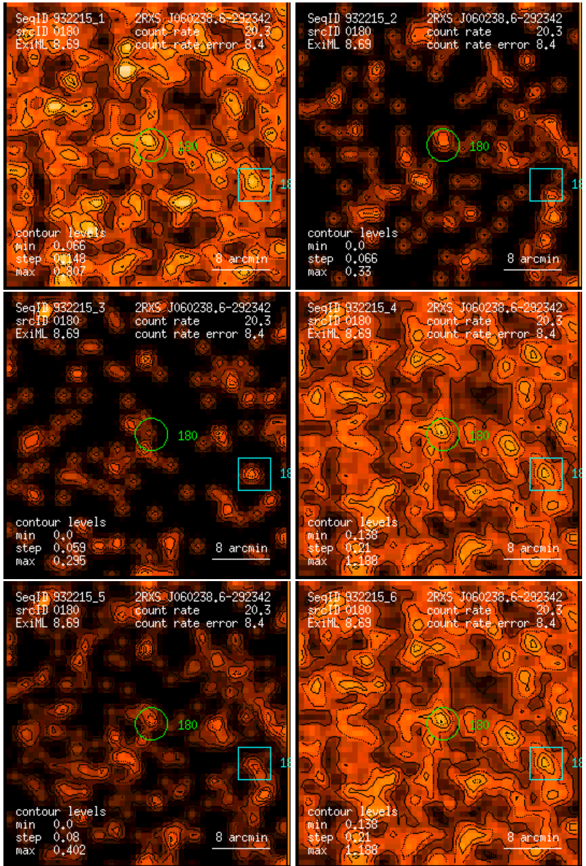
Figure 180: RASS 932215: detection 0180: band rate images, Gaussian filter: (1) PSPC channels 11 – 41, (2) 52 – 90, (3) 91 – 201, (4) 11 – 235, (5) 52 – 201, (6) 11 – 201. Broad band rates in counts/ks. Band rate contour levels in counts/ks/arcmin 2 .
