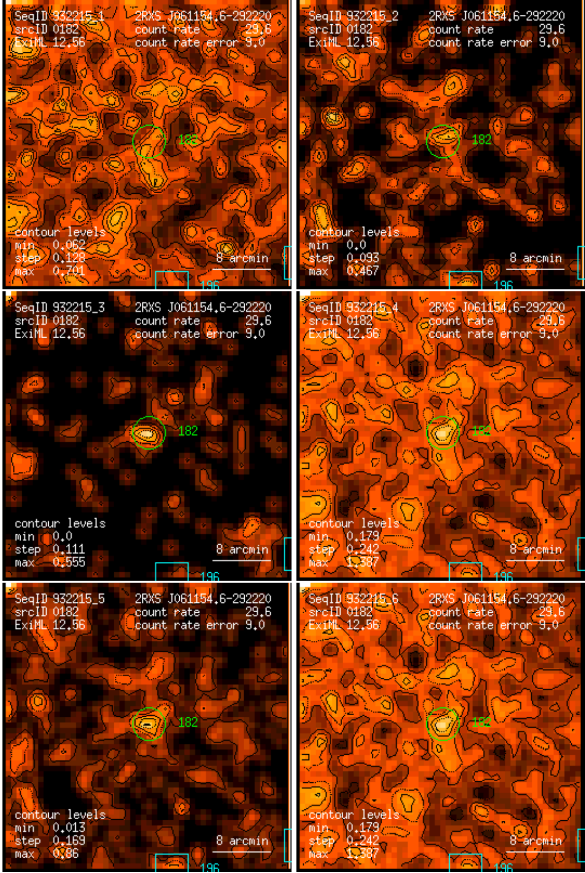
Figure 182: RASS 932215: detection 0182: band rate images, Gaussian filter: (1) PSPC channels 11 – 41, (2) 52 – 90, (3) 91 – 201, (4) 11 – 235, (5) 52 – 201, (6) 11 – 201. Broad band rates in counts/ks. Band rate contour levels in counts/ks/arcmin 2 .
