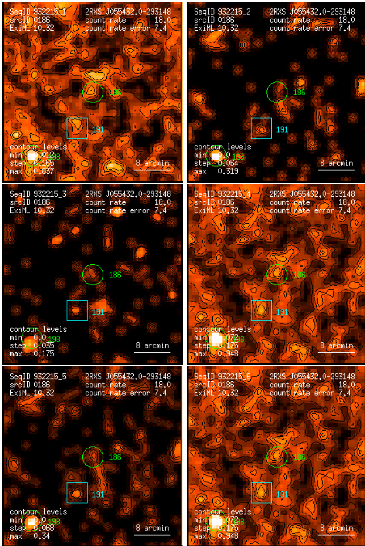
Figure 186: RASS 932215: detection 0186: band rate images, Gaussian filter: (1) PSPC channels 11 – 41, (2) 52 – 90, (3) 91 – 201, (4) 11 – 235, (5) 52 – 201, (6) 11 – 201. Broad band rates in counts/ks. Band rate contour levels in counts/ks/arcmin 2 .
