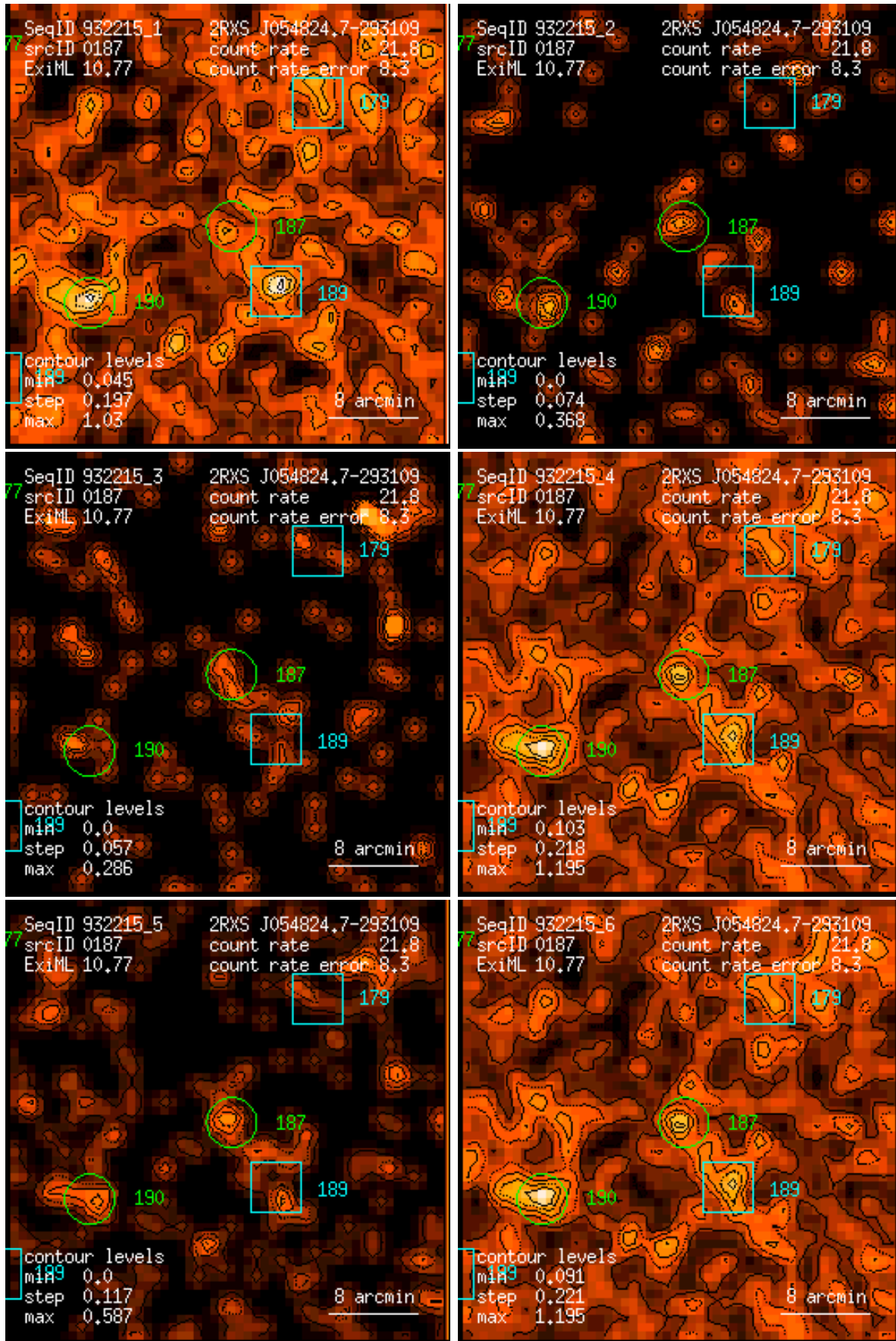
Figure 187: RASS 932215: detection 0187: band rate images, Gaussian filter: (1) PSPC channels 11 – 41, (2) 52 – 90, (3) 91 – 201, (4) 11 – 235, (5) 52 – 201, (6) 11 – 201. Broad band rates in counts/ks. Band rate contour levels in counts/ks/arcmin 2 .
