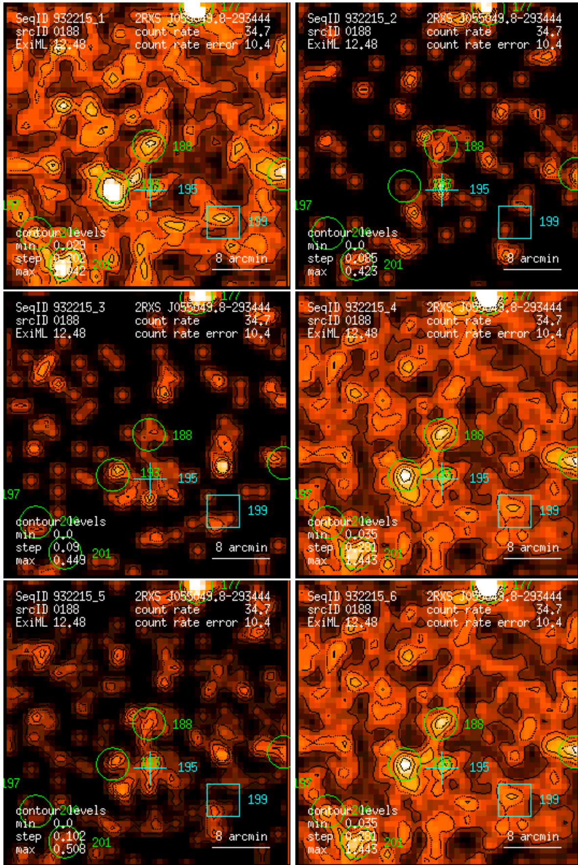
Figure 188: RASS 932215: detection 0188: band rate images, Gaussian filter: (1) PSPC channels 11 – 41, (2) 52 – 90, (3) 91 – 201, (4) 11 – 235, (5) 52 – 201, (6) 11 – 201. Broad band rates in counts/ks. Band rate contour levels in counts/ks/arcmin 2 .
