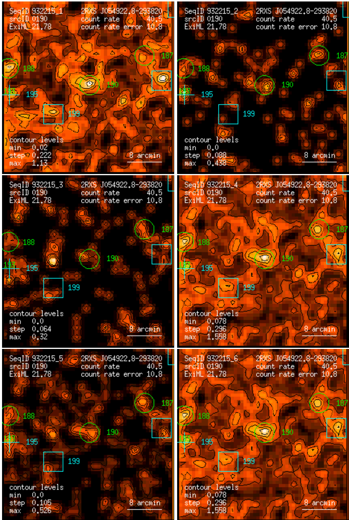
Figure 190: RASS 932215: detection 0190: band rate images, Gaussian filter: (1) PSPC channels 11 – 41, (2) 52 – 90, (3) 91 – 201, (4) 11 – 235, (5) 52 – 201, (6) 11 – 201. Broad band rates in counts/ks. Band rate contour levels in counts/ks/arcmin 2 .
