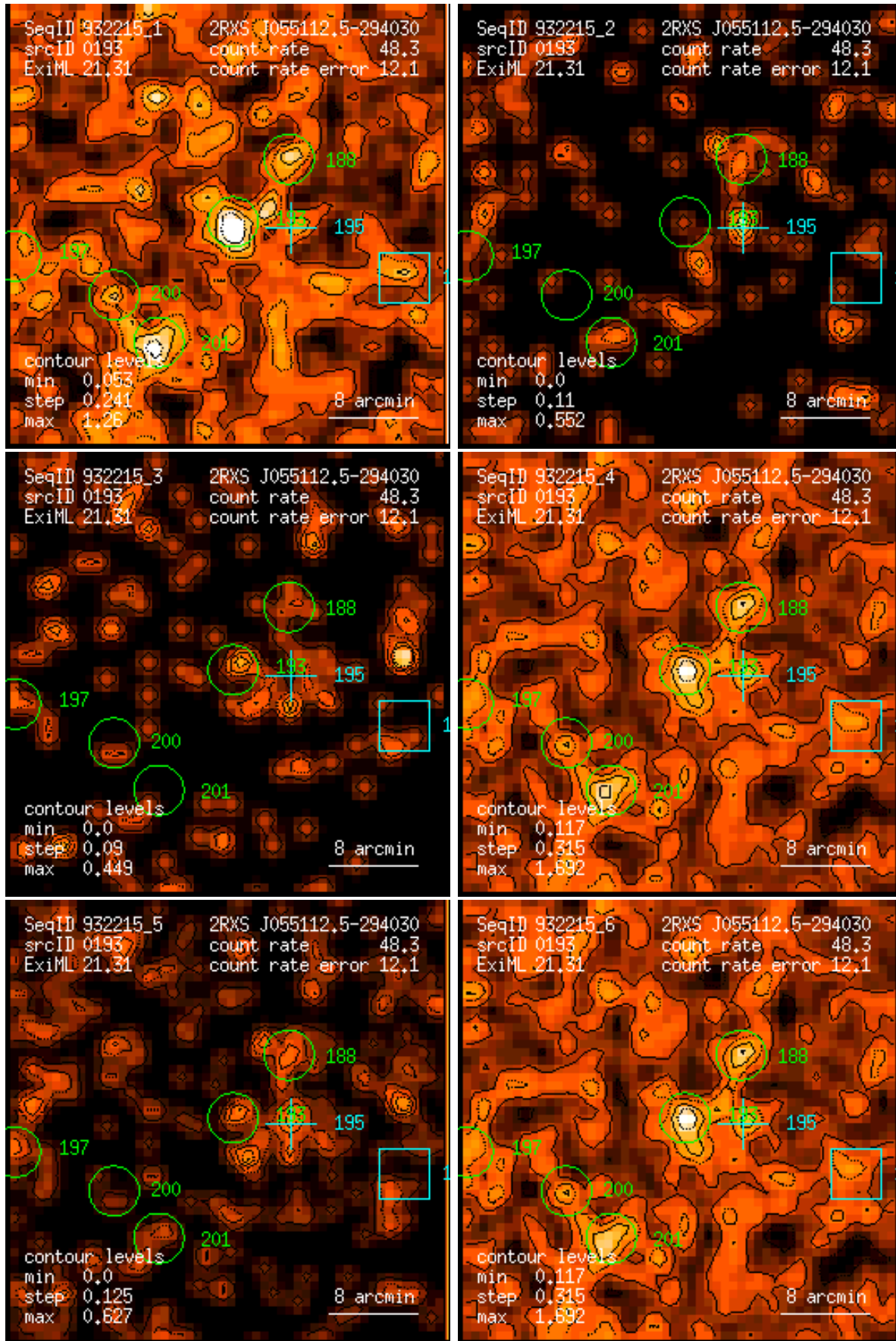
Figure 193: RASS 932215: detection 0193: band rate images, Gaussian filter: (1) PSPC channels 11 – 41, (2) 52 – 90, (3) 91 – 201, (4) 11 – 235, (5) 52 – 201, (6) 11 – 201. Broad band rates in counts/ks. Band rate contour levels in counts/ks/arcmin 2 .
