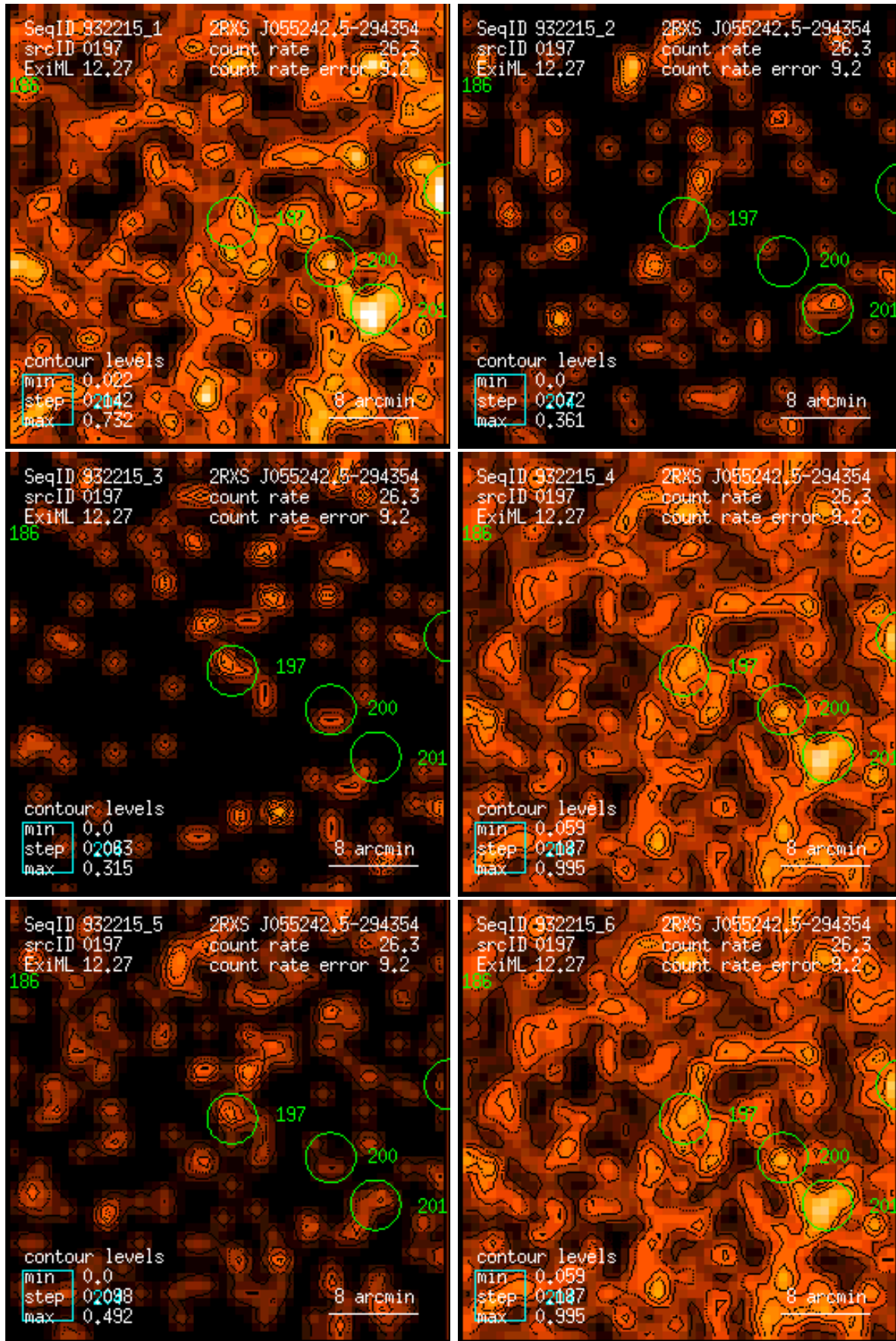
Figure 197: RASS 932215: detection 0197: band rate images, Gaussian filter: (1) PSPC channels 11 – 41, (2) 52 – 90, (3) 91 – 201, (4) 11 – 235, (5) 52 – 201, (6) 11 – 201. Broad band rates in counts/ks. Band rate contour levels in counts/ks/arcmin 2 .
