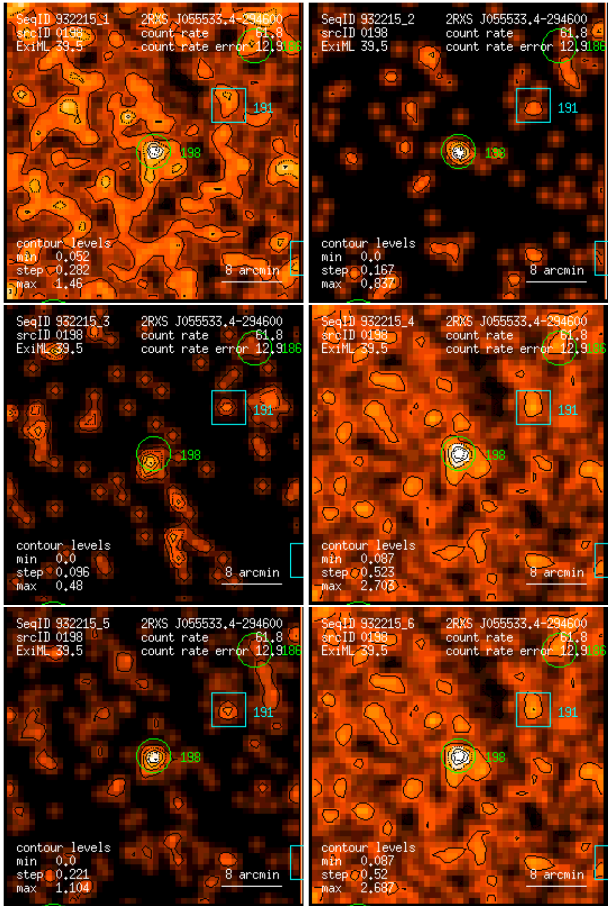
Figure 198: RASS 932215: detection 0198: band rate images, Gaussian filter: (1) PSPC channels 11 – 41, (2) 52 – 90, (3) 91 – 201, (4) 11 – 235, (5) 52 – 201, (6) 11 – 201. Broad band rates in counts/ks. Band rate contour levels in counts/ks/arcmin 2 .
