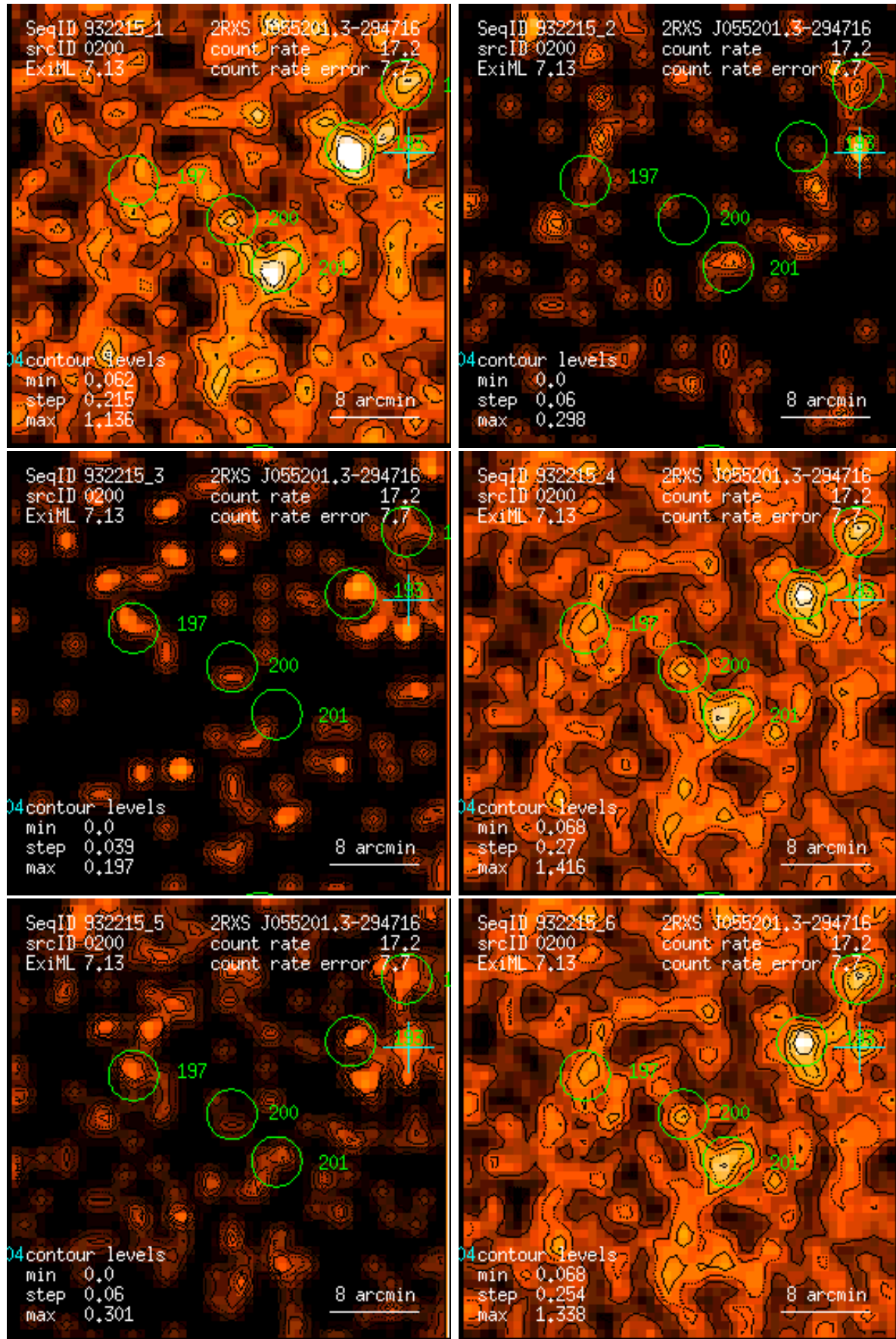
Figure 200: RASS 932215: detection 0200: band rate images, Gaussian filter: (1) PSPC channels 11 – 41, (2) 52 – 90, (3) 91 – 201, (4) 11 – 235, (5) 52 – 201, (6) 11 – 201. Broad band rates in counts/ks. Band rate contour levels in counts/ks/arcmin 2 .
