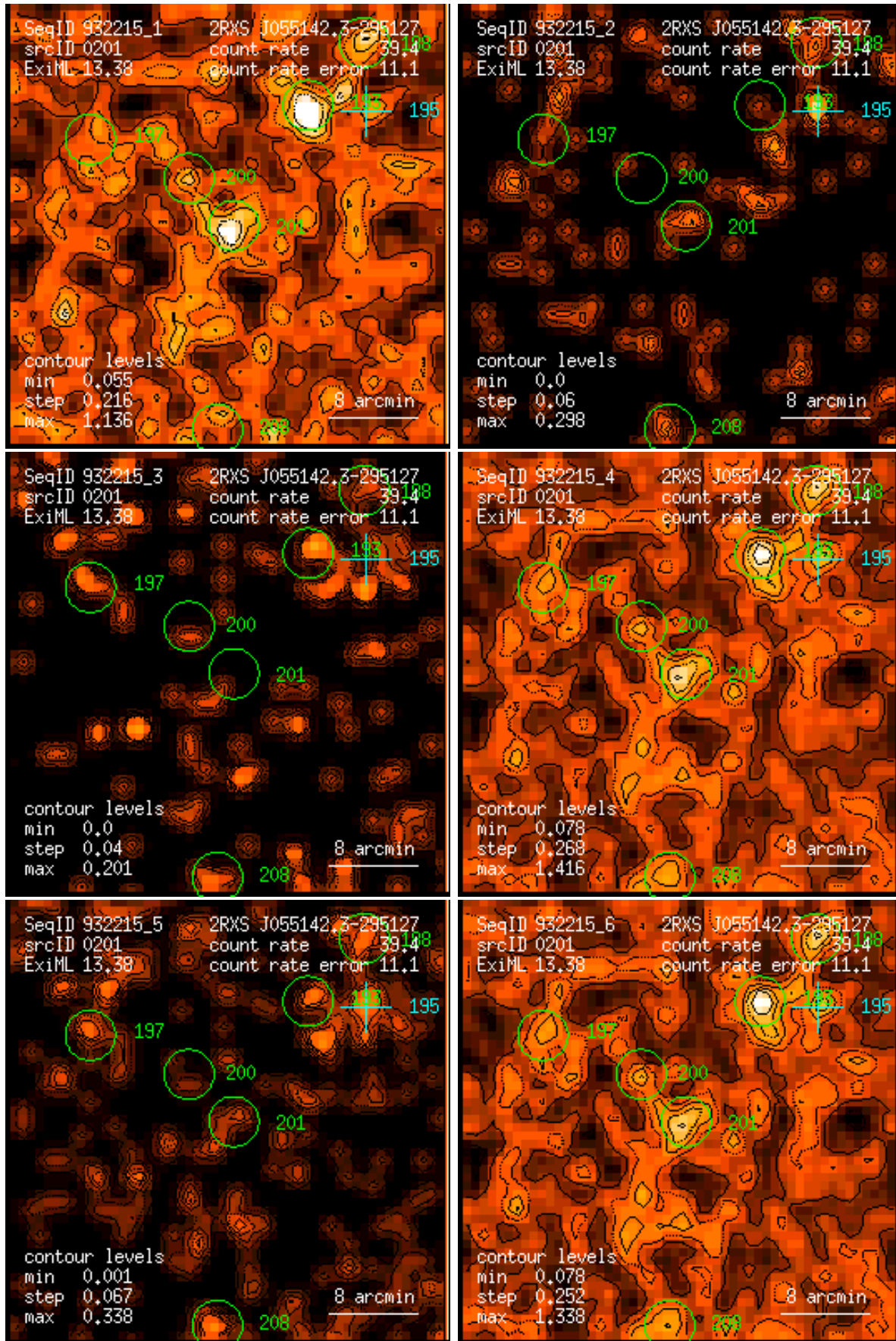
Figure 201: RASS 932215: detection 0201: band rate images, Gaussian filter: (1) PSPC channels 11 – 41, (2) 52 – 90, (3) 91 – 201, (4) 11 – 235, (5) 52 – 201, (6) 11 – 201. Broad band rates in counts/ks. Band rate contour levels in counts/ks/arcmin 2 .
