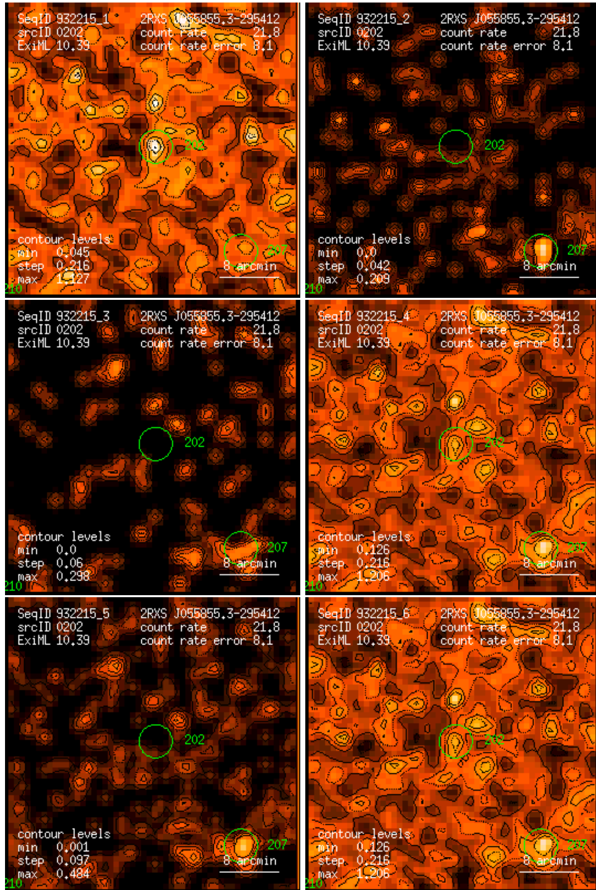
Figure 202: RASS 932215: detection 0202: band rate images, Gaussian filter: (1) PSPC channels 11 – 41, (2) 52 – 90, (3) 91 – 201, (4) 11 – 235, (5) 52 – 201, (6) 11 – 201. Broad band rates in counts/ks. Band rate contour levels in counts/ks/arcmin 2 .
