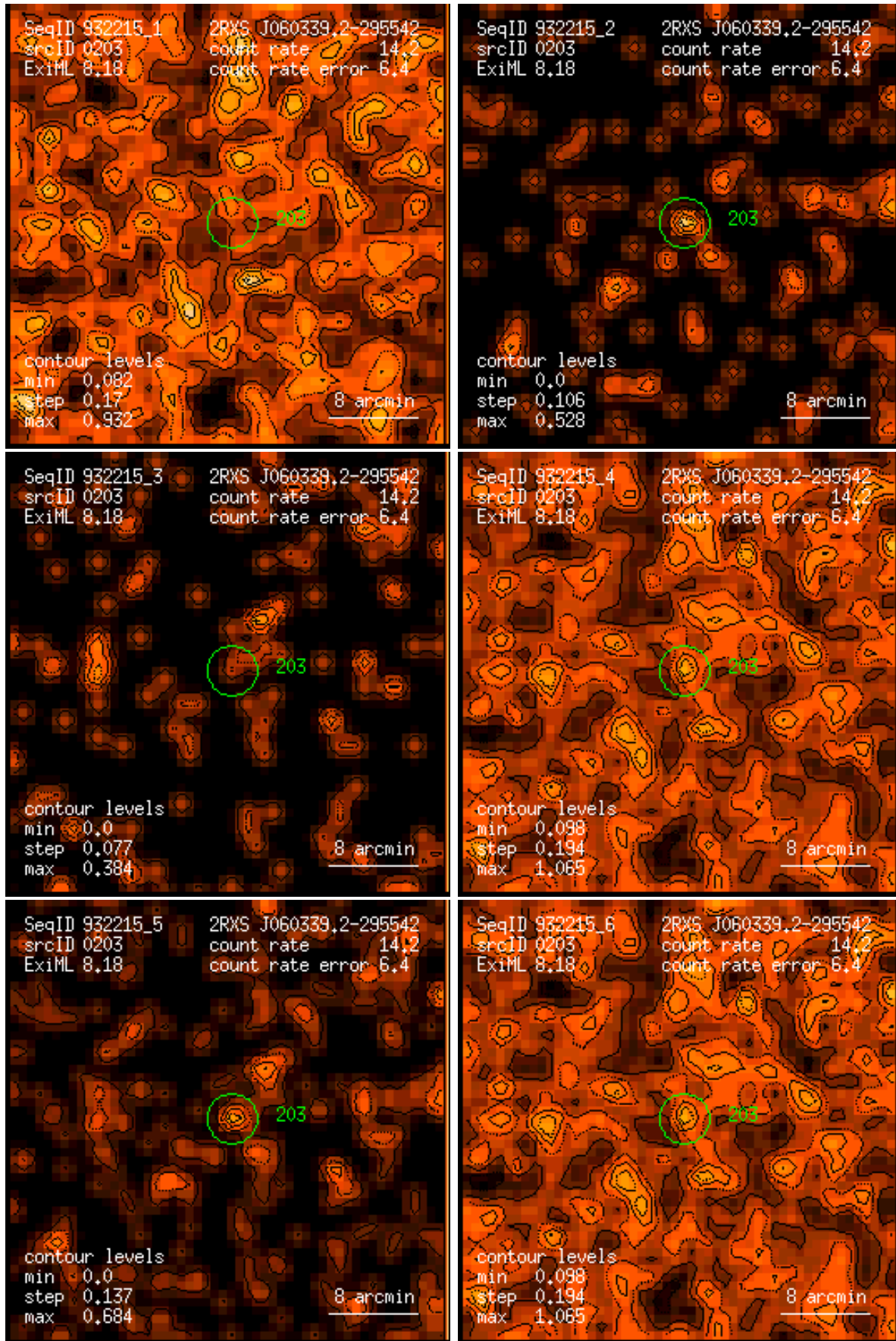
Figure 203: RASS 932215: detection 0203: band rate images, Gaussian filter: (1) PSPC channels 11 – 41, (2) 52 – 90, (3) 91 – 201, (4) 11 – 235, (5) 52 – 201, (6) 11 – 201. Broad band rates in counts/ks. Band rate contour levels in counts/ks/arcmin 2 .
