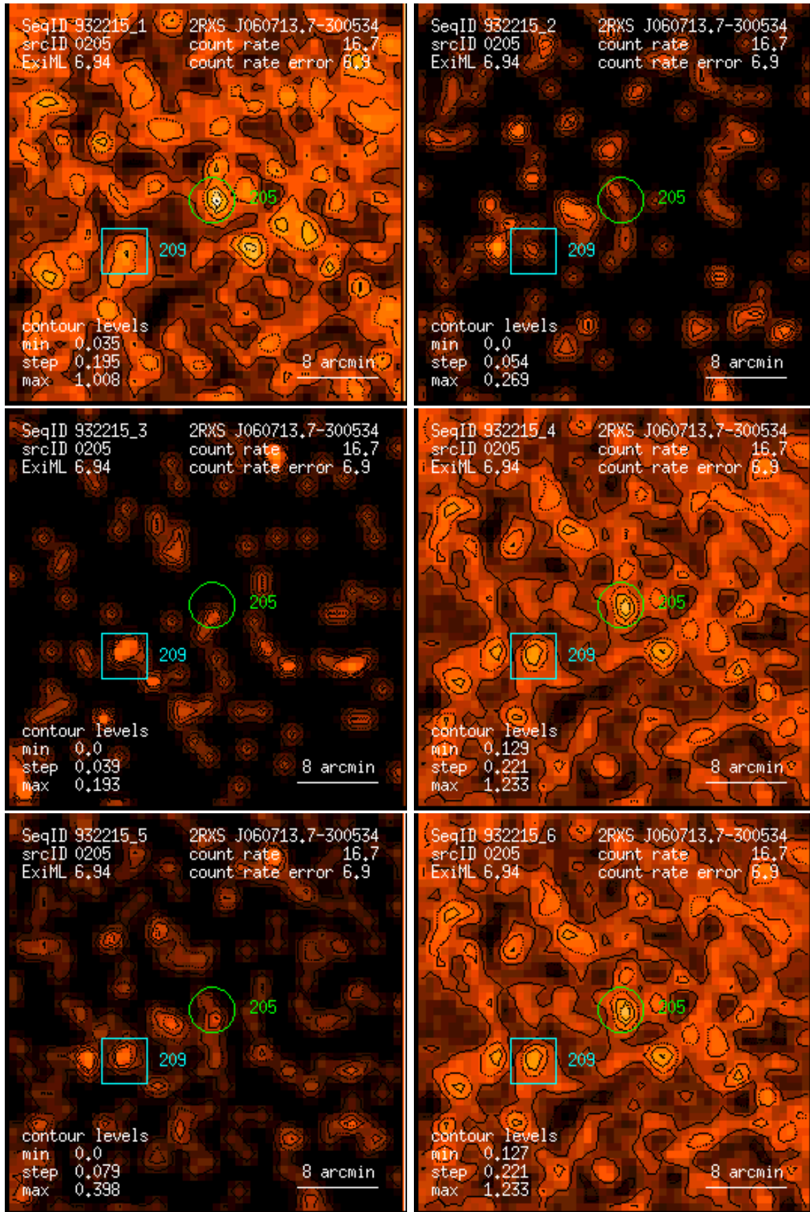
Figure 205: RASS 932215: detection 0205: band rate images, Gaussian filter: (1) PSPC channels 11 – 41, (2) 52 – 90, (3) 91 – 201, (4) 11 – 235, (5) 52 – 201, (6) 11 – 201. Broad band rates in counts/ks. Band rate contour levels in counts/ks/arcmin 2 .
