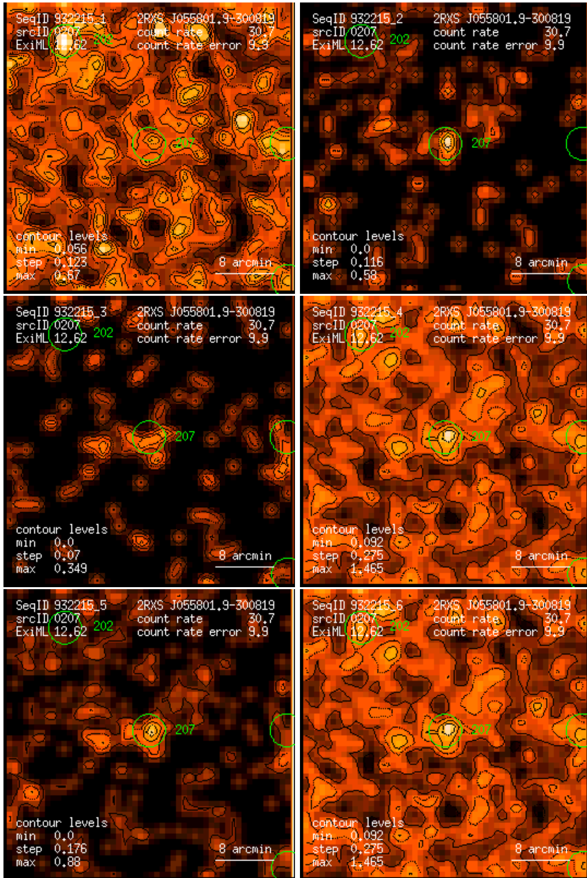
Figure 207: RASS 932215: detection 0207: band rate images, Gaussian filter: (1) PSPC channels 11 – 41, (2) 52 – 90, (3) 91 – 201, (4) 11 – 235, (5) 52 – 201, (6) 11 – 201. Broad band rates in counts/ks. Band rate contour levels in counts/ks/arcmin 2 .
