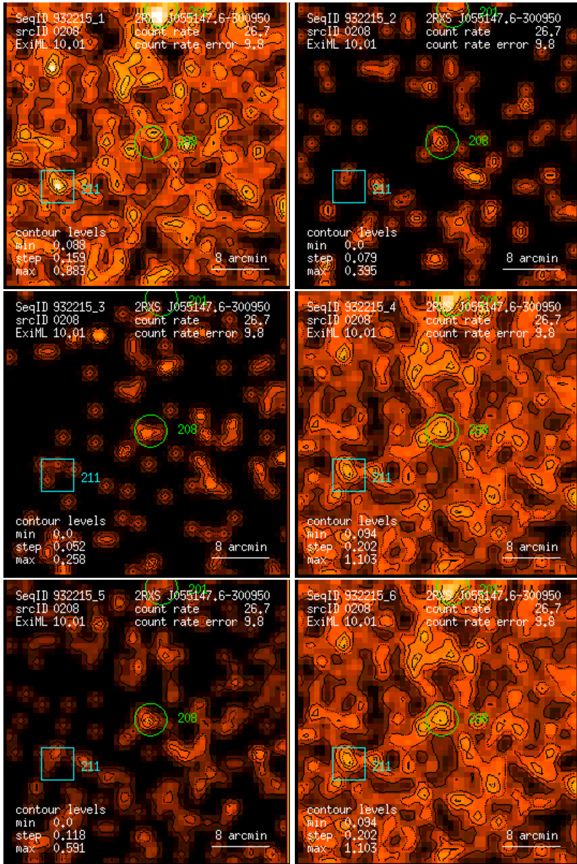
Figure 208: RASS 932215: detection 0208: band rate images, Gaussian filter: (1) PSPC channels 11 – 41, (2) 52 – 90, (3) 91 – 201, (4) 11 – 235, (5) 52 – 201, (6) 11 – 201. Broad band rates in counts/ks. Band rate contour levels in counts/ks/arcmin 2 .
