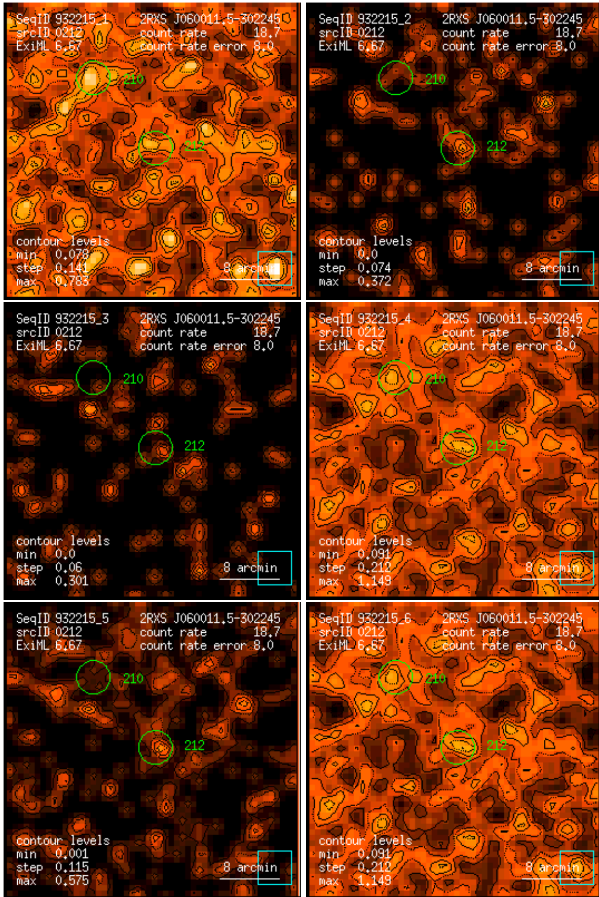
Figure 212: RASS 932215: detection 0212: band rate images, Gaussian filter: (1) PSPC channels 11 – 41, (2) 52 – 90, (3) 91 – 201, (4) 11 – 235, (5) 52 – 201, (6) 11 – 201. Broad band rates in counts/ks. Band rate contour levels in counts/ks/arcmin 2 .
