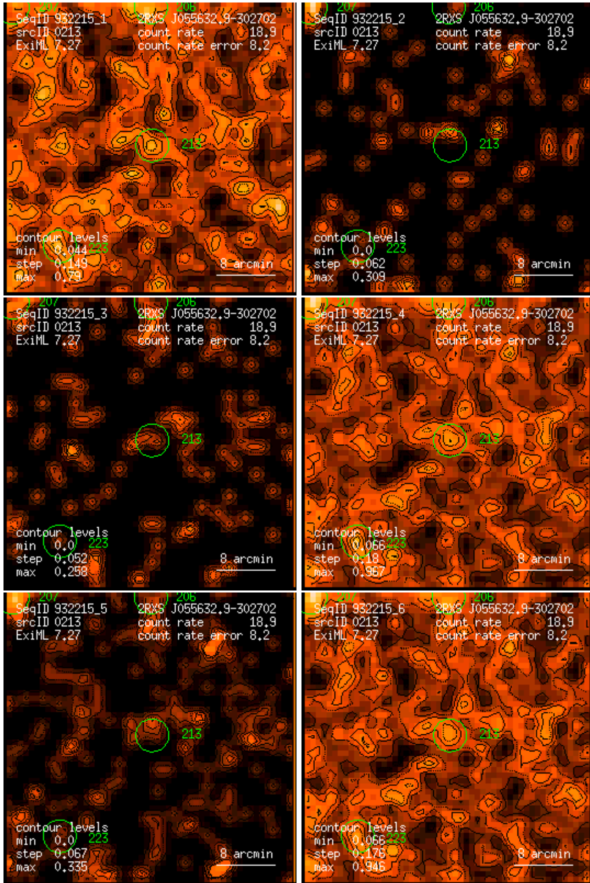
Figure 213: RASS 932215: detection 0213: band rate images, Gaussian filter: (1) PSPC channels 11 – 41, (2) 52 – 90, (3) 91 – 201, (4) 11 – 235, (5) 52 – 201, (6) 11 – 201. Broad band rates in counts/ks. Band rate contour levels in counts/ks/arcmin 2 .
