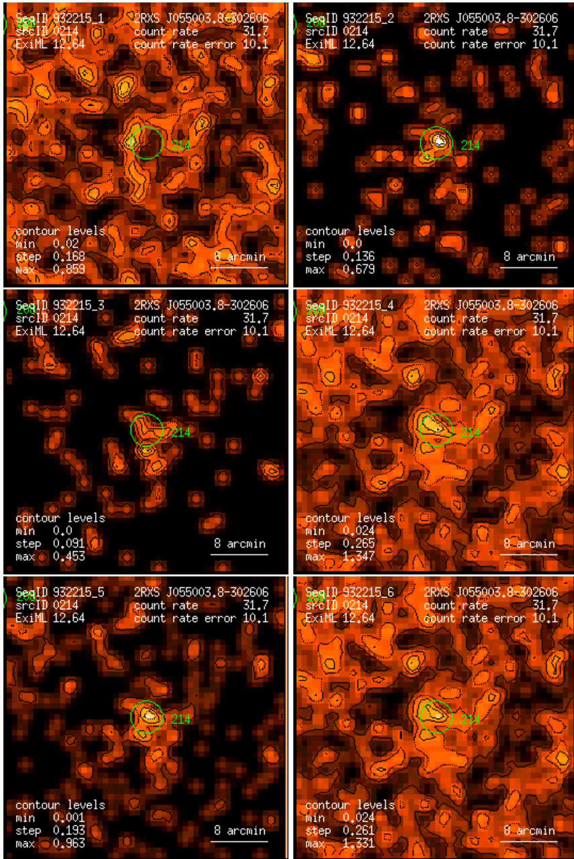
Figure 214: RASS 932215: detection 0214: band rate images, Gaussian filter: (1) PSPC channels 11 – 41, (2) 52 – 90, (3) 91 – 201, (4) 11 – 235, (5) 52 – 201, (6) 11 – 201. Broad band rates in counts/ks. Band rate contour levels in counts/ks/arcmin 2 .
