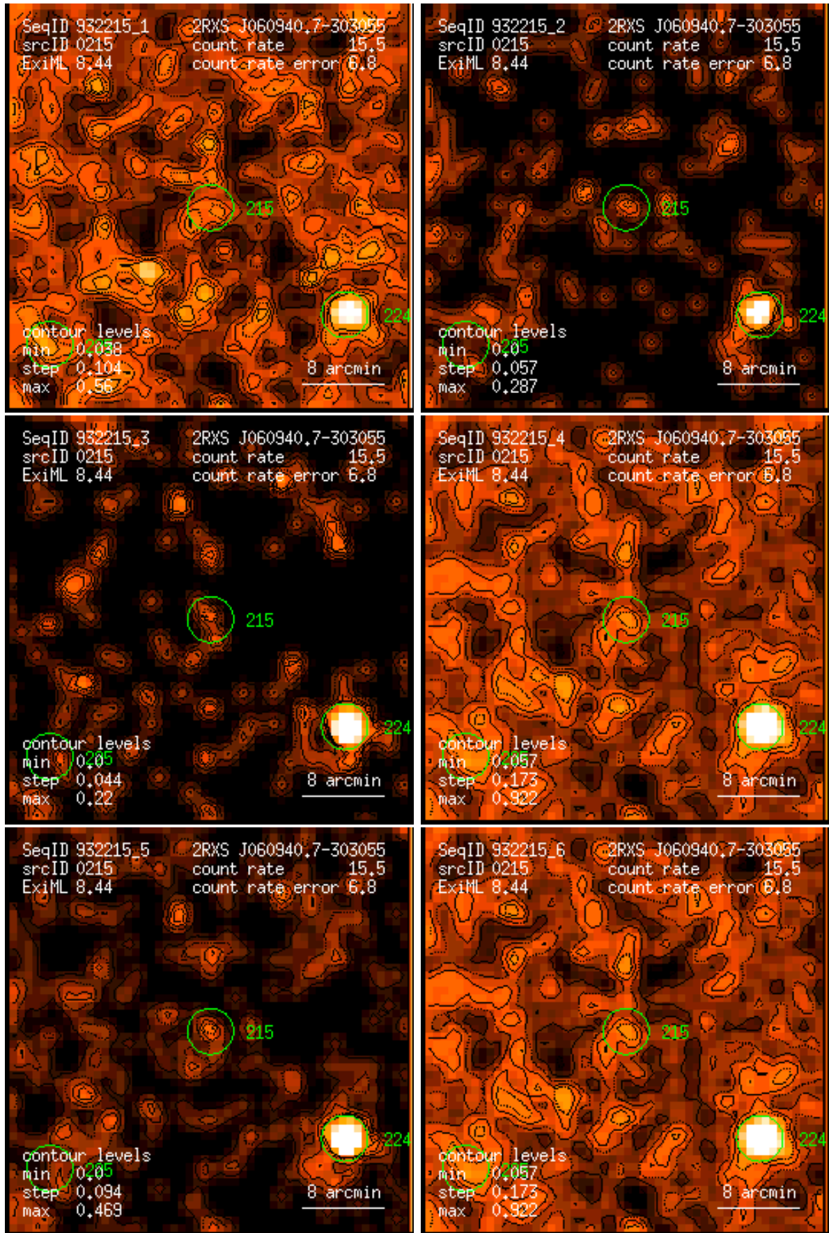
Figure 215: RASS 932215: detection 0215: band rate images, Gaussian filter: (1) PSPC channels 11 – 41, (2) 52 – 90, (3) 91 – 201, (4) 11 – 235, (5) 52 – 201, (6) 11 – 201. Broad band rates in counts/ks. Band rate contour levels in counts/ks/arcmin 2 .
