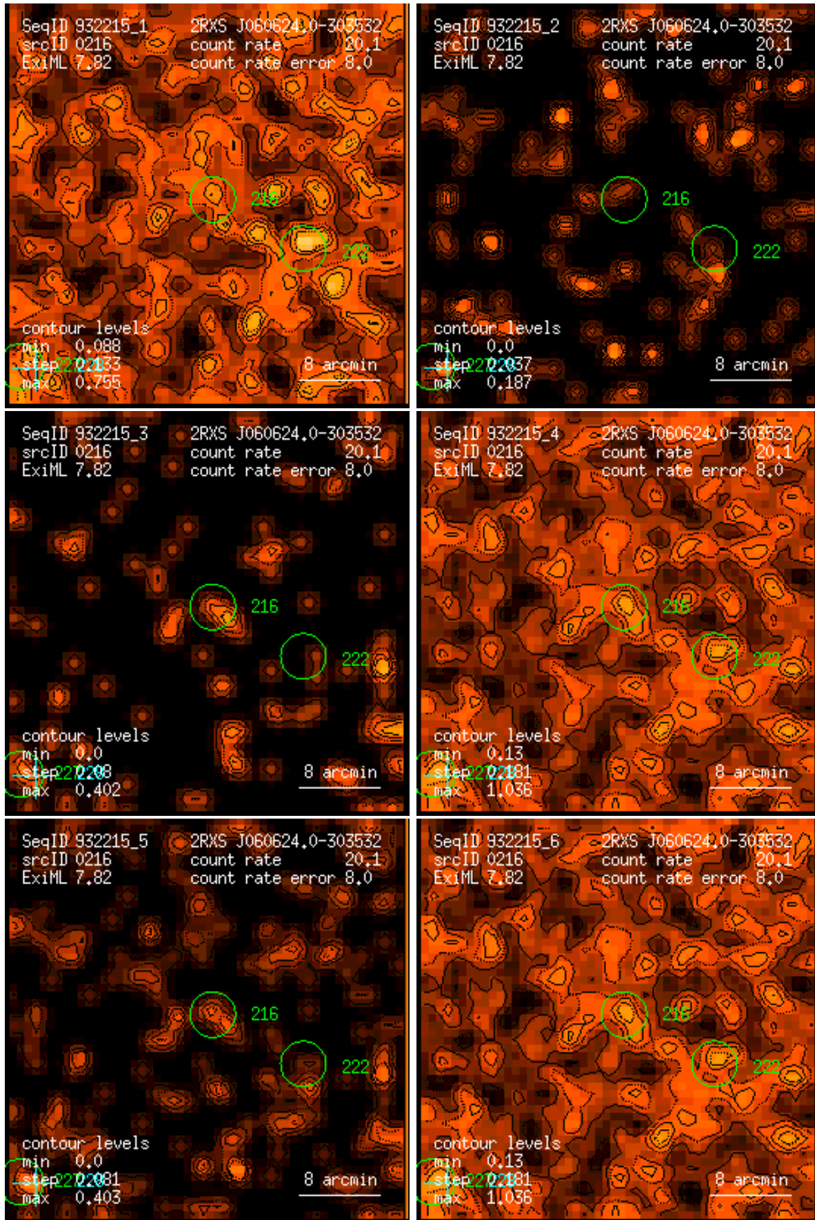
Figure 216: RASS 932215: detection 0216: band rate images, Gaussian filter: (1) PSPC channels 11 – 41, (2) 52 – 90, (3) 91 – 201, (4) 11 – 235, (5) 52 – 201, (6) 11 – 201. Broad band rates in counts/ks. Band rate contour levels in counts/ks/arcmin 2 .
