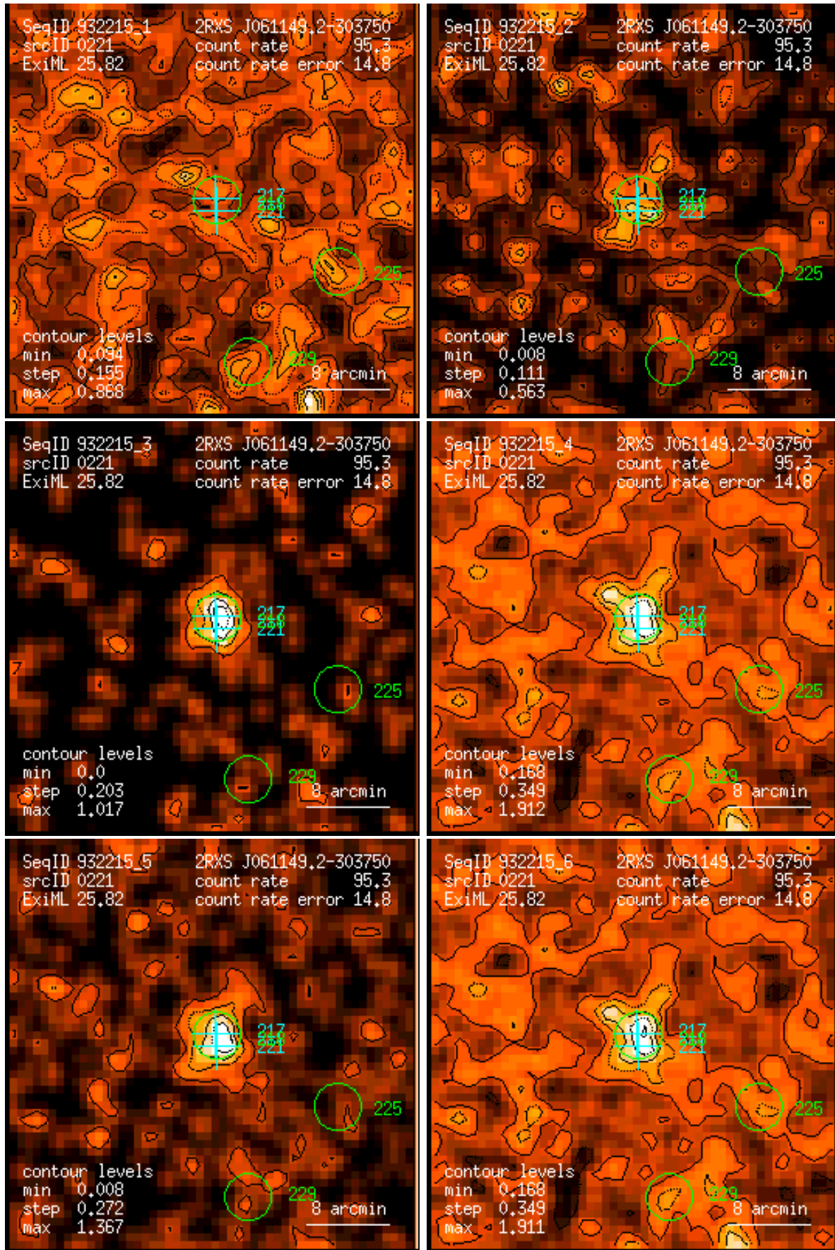
Figure 221: RASS 932215: detection 0221: band rate images, Gaussian filter: (1) PSPC channels 11 – 41, (2) 52 – 90, (3) 91 – 201, (4) 11 – 235, (5) 52 – 201, (6) 11 – 201. Broad band rates in counts/ks. Band rate contour levels in counts/ks/arcmin 2 .
