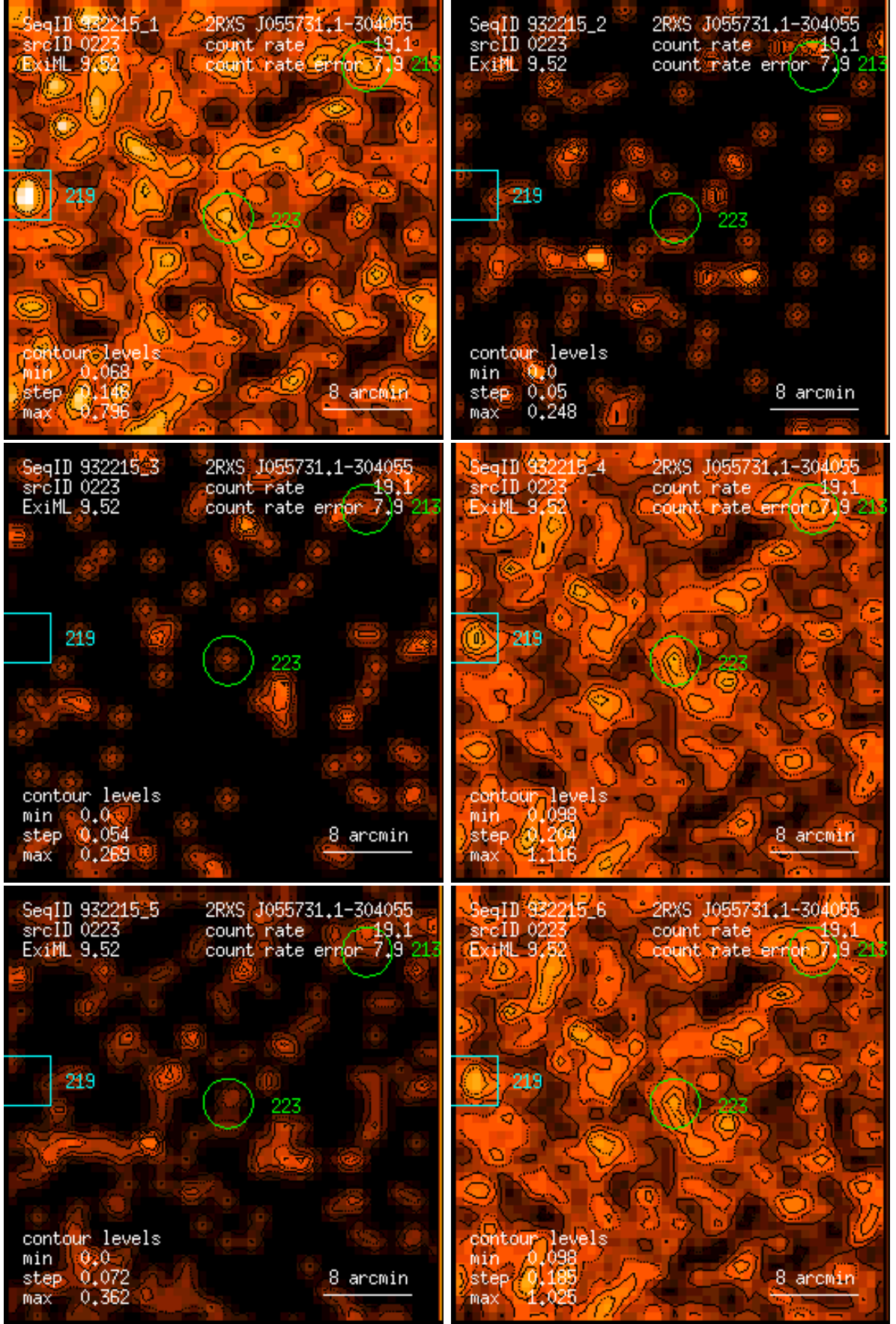
Figure 223: RASS 932215: detection 0223: band rate images, Gaussian filter: (1) PSPC channels 11 – 41, (2) 52 – 90, (3) 91 – 201, (4) 11 – 235, (5) 52 – 201, (6) 11 – 201. Broad band rates in counts/ks. Band rate contour levels in counts/ks/arcmin 2 .
