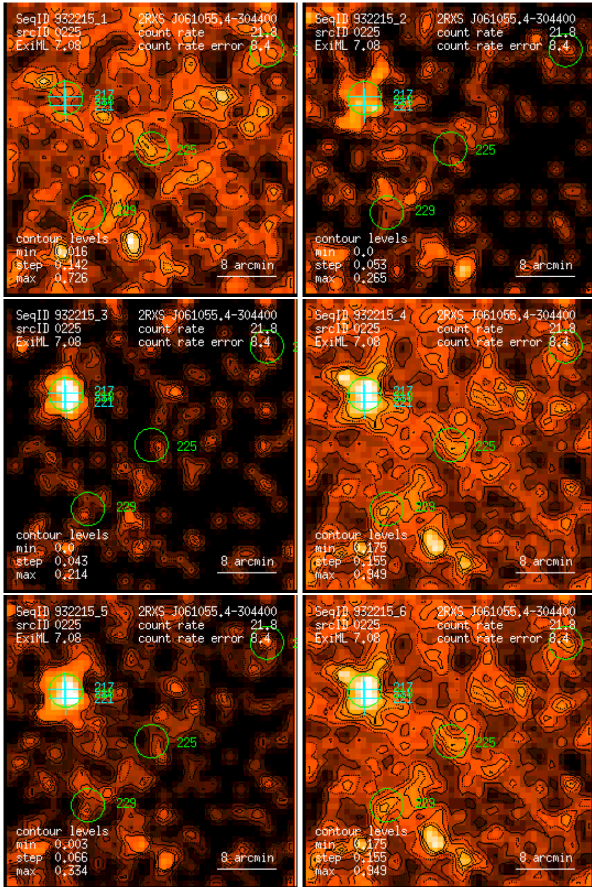
Figure 225: RASS 932215: detection 0225: band rate images, Gaussian filter: (1) PSPC channels 11 – 41, (2) 52 – 90, (3) 91 – 201, (4) 11 – 235, (5) 52 – 201, (6) 11 – 201. Broad band rates in counts/ks. Band rate contour levels in counts/ks/arcmin 2 .
