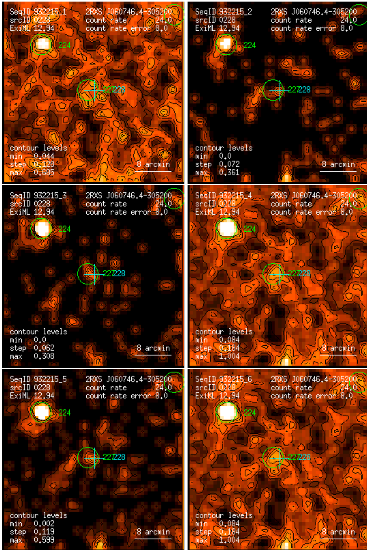
Figure 228: RASS 932215: detection 0228: band rate images, Gaussian filter: (1) PSPC channels 11 – 41, (2) 52 – 90, (3) 91 – 201, (4) 11 – 235, (5) 52 – 201, (6) 11 – 201. Broad band rates in counts/ks. Band rate contour levels in counts/ks/arcmin 2 .
