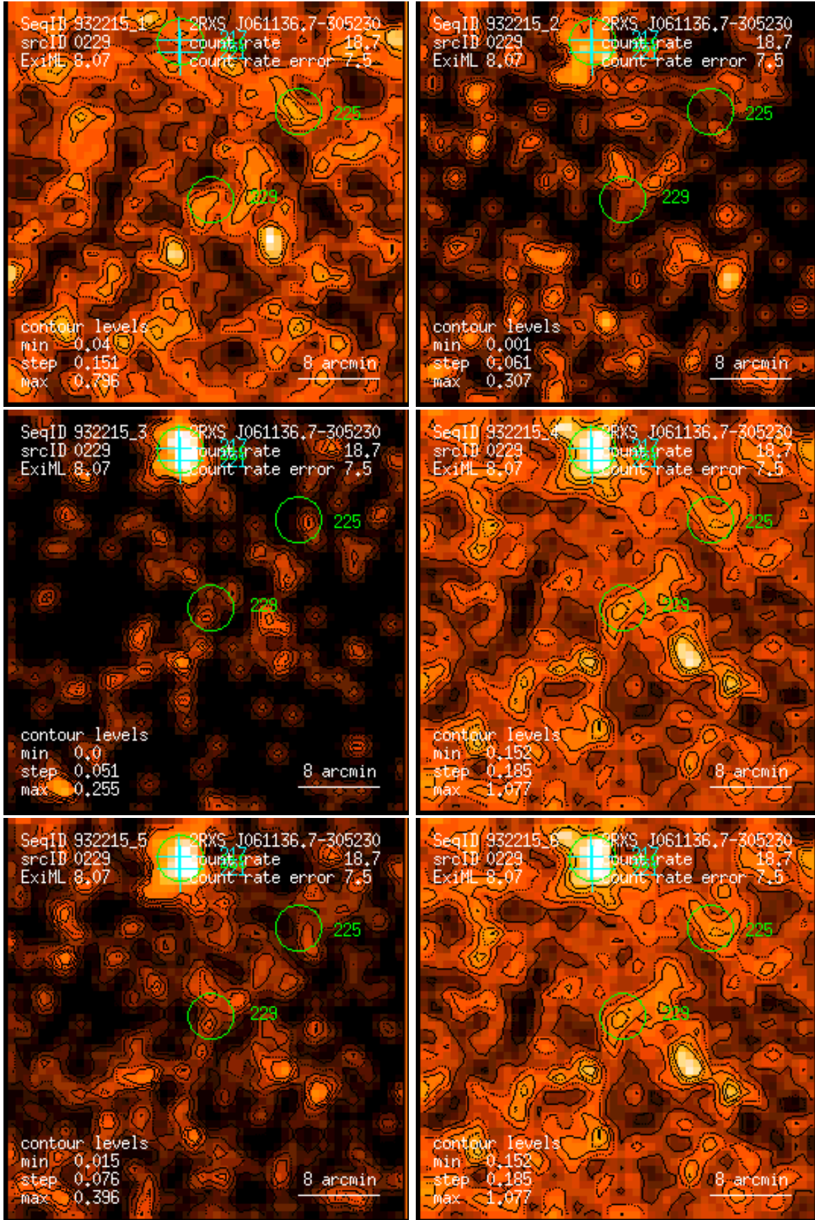
Figure 229: RASS 932215: detection 0229: band rate images, Gaussian filter: (1) PSPC channels 11 – 41, (2) 52 – 90, (3) 91 – 201, (4) 11 – 235, (5) 52 – 201, (6) 11 – 201. Broad band rates in counts/ks. Band rate contour levels in counts/ks/arcmin 2 .
