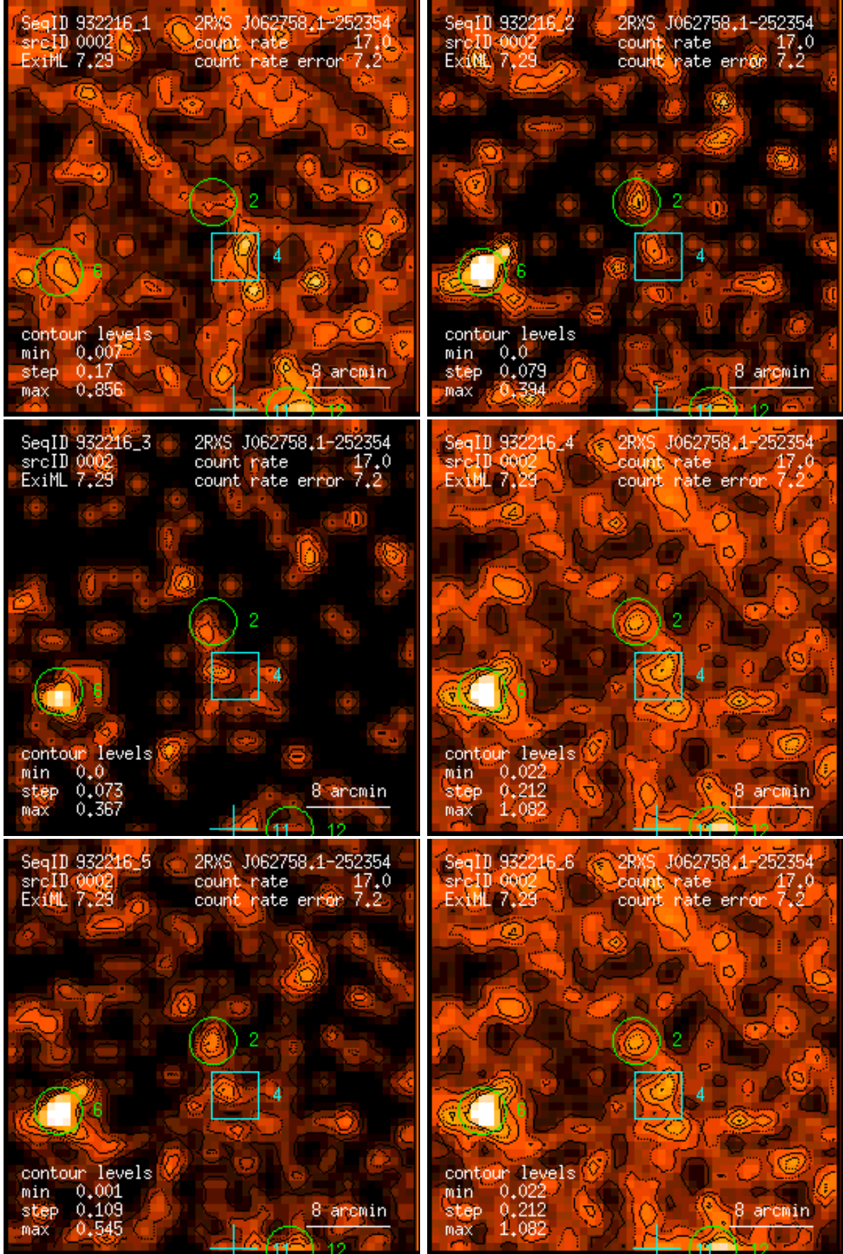
Figure 2: RASS 932216: detection 0002: band rate images, Gaussian filter: (1) PSPC channels 11 – 41, (2) 52 – 90, (3) 91 – 201, (4) 11 – 235, (5) 52 – 201, (6) 11 – 201. Broad band rates in counts/ks. Band rate contour levels in counts/ks/arcmin 2 .
