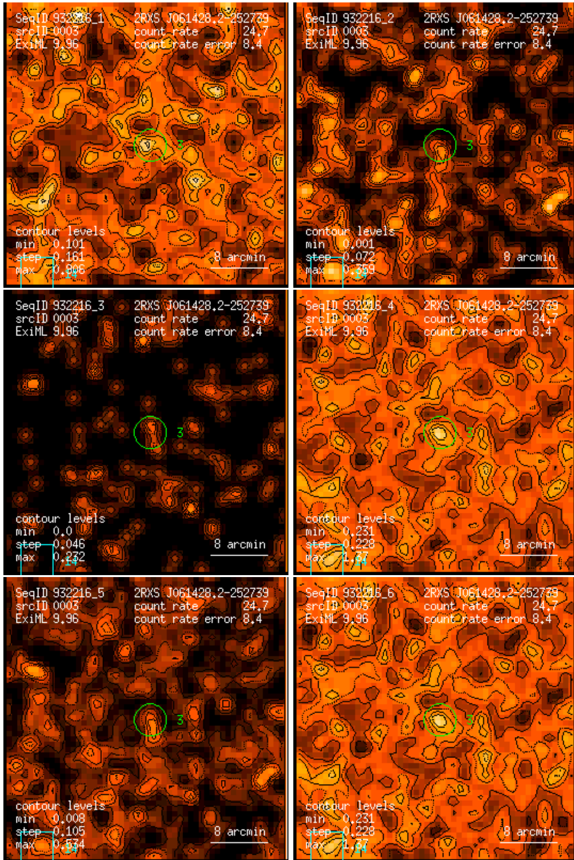
Figure 3: RASS 932216: detection 0003: band rate images, Gaussian filter: (1) PSPC channels 11 – 41, (2) 52 – 90, (3) 91 – 201, (4) 11 – 235, (5) 52 – 201, (6) 11 – 201. Broad band rates in counts/ks. Band rate contour levels in counts/ks/arcmin 2 .
