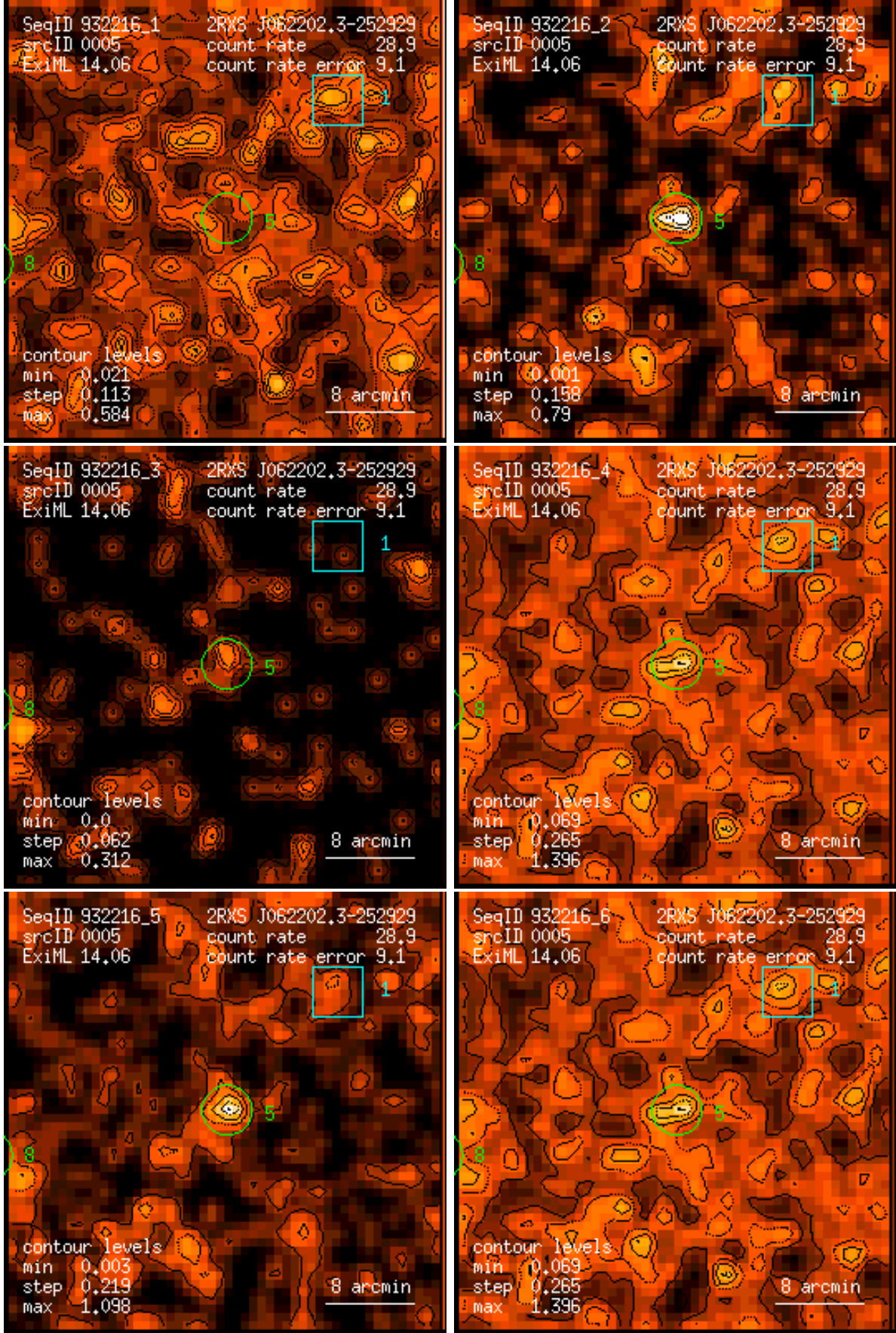
Figure 5: RASS 932216: detection 0005: band rate images, Gaussian filter: (1) PSPC channels 11 – 41, (2) 52 – 90, (3) 91 – 201, (4) 11 – 235, (5) 52 – 201, (6) 11 – 201. Broad band rates in counts/ks. Band rate contour levels in counts/ks/arcmin 2 .
