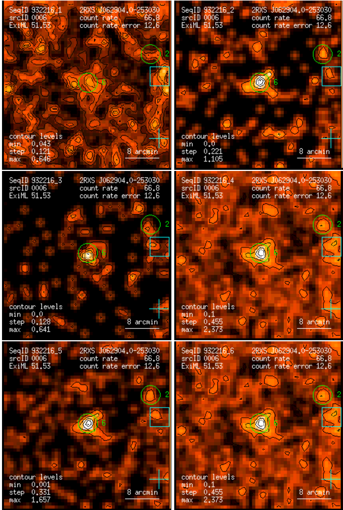
Figure 6: RASS 932216: detection 0006: band rate images, Gaussian filter: (1) PSPC channels 11 – 41, (2) 52 – 90, (3) 91 – 201, (4) 11 – 235, (5) 52 – 201, (6) 11 – 201. Broad band rates in counts/ks. Band rate contour levels in counts/ks/arcmin 2 .
