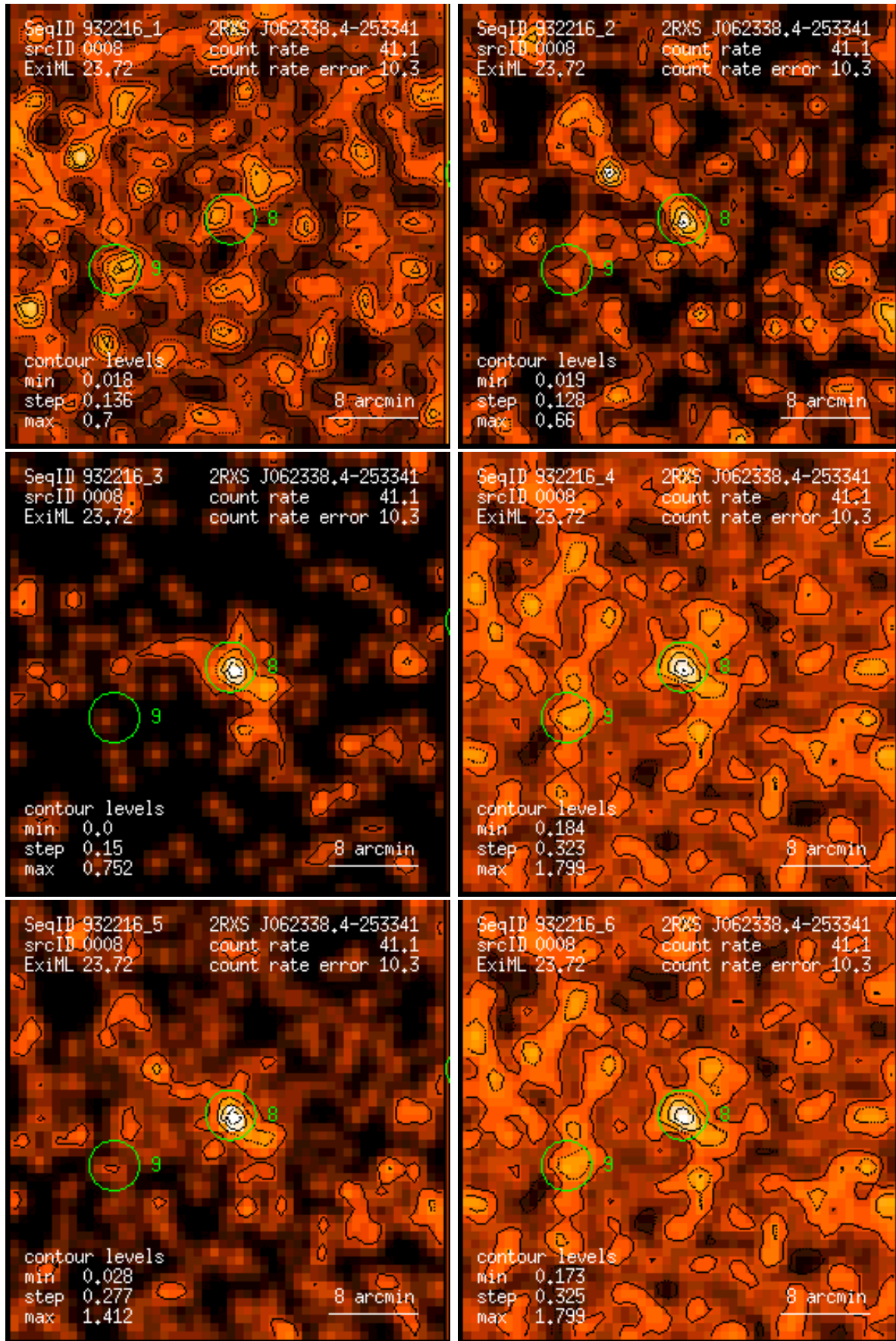
Figure 8: RASS 932216: detection 0008: band rate images, Gaussian filter: (1) PSPC channels 11 – 41, (2) 52 – 90, (3) 91 – 201, (4) 11 – 235, (5) 52 – 201, (6) 11 – 201. Broad band rates in counts/ks. Band rate contour levels in counts/ks/arcmin 2 .
