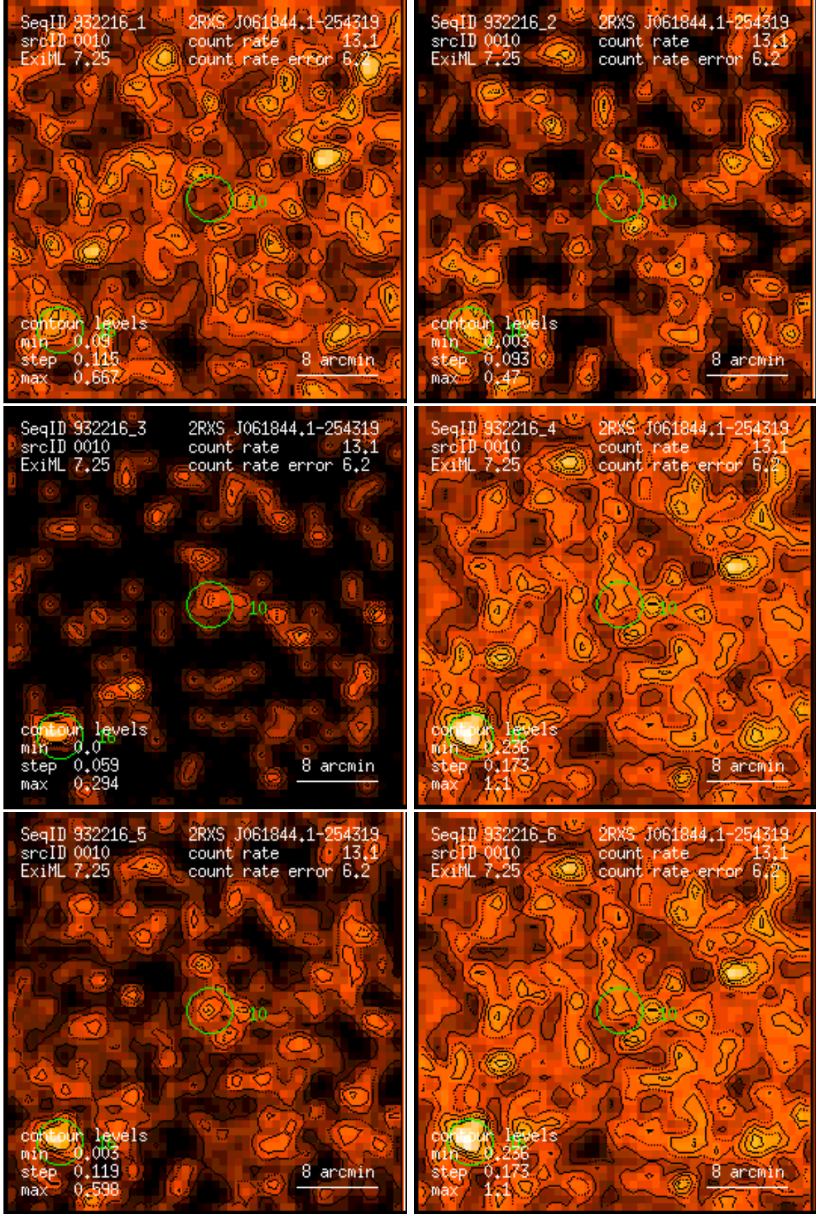
Figure 10: RASS 932216: detection 0010: band rate images, Gaussian filter: (1) PSPC channels 11 – 41, (2) 52 – 90, (3) 91 – 201, (4) 11 – 235, (5) 52 – 201, (6) 11 – 201. Broad band rates in counts/ks. Band rate contour levels in counts/ks/arcmin 2 .
