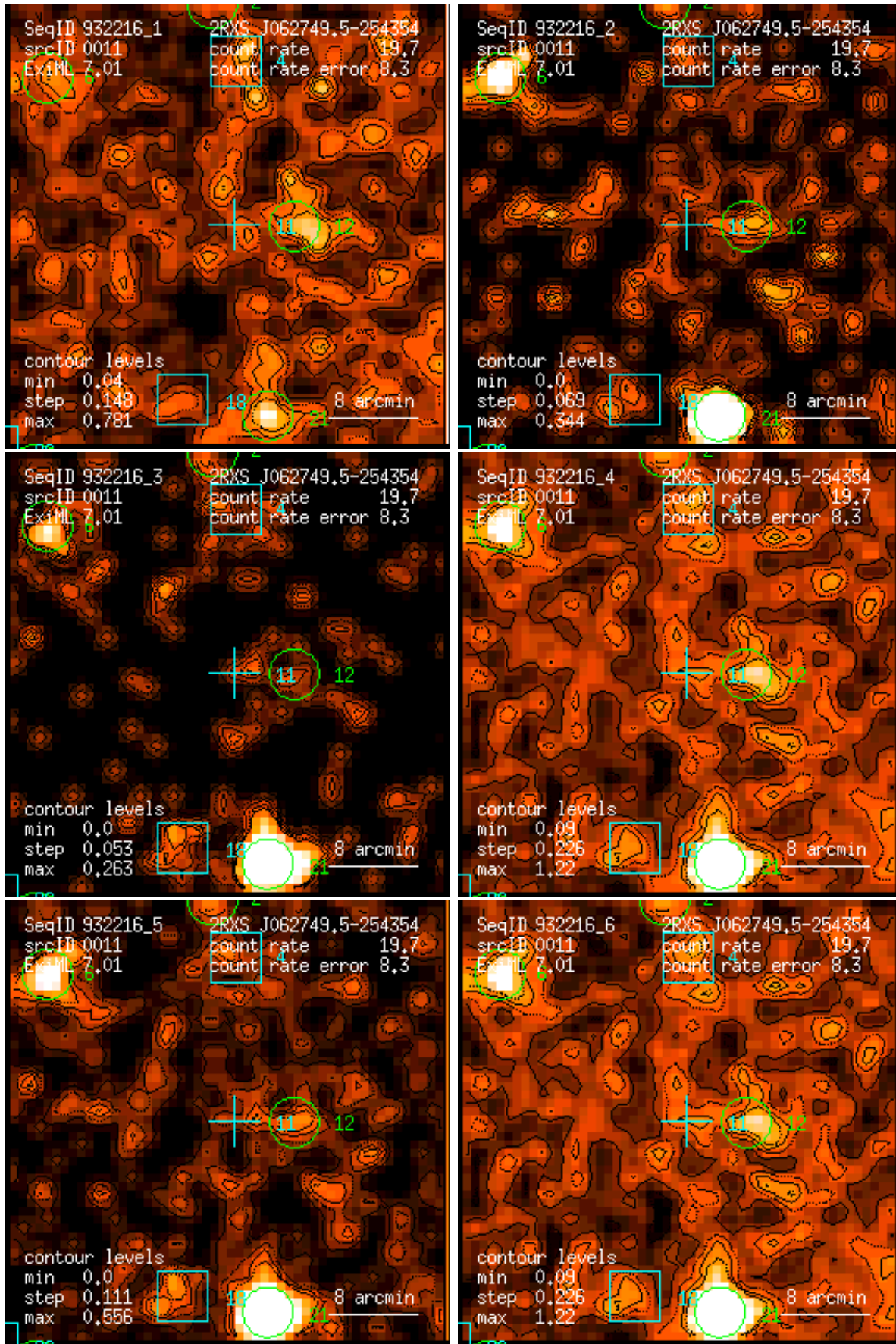
Figure 11: RASS 932216: detection 0011: band rate images, Gaussian filter: (1) PSPC channels 11 – 41, (2) 52 – 90, (3) 91 – 201, (4) 11 – 235, (5) 52 – 201, (6) 11 – 201. Broad band rates in counts/ks. Band rate contour levels in counts/ks/arcmin 2 .
