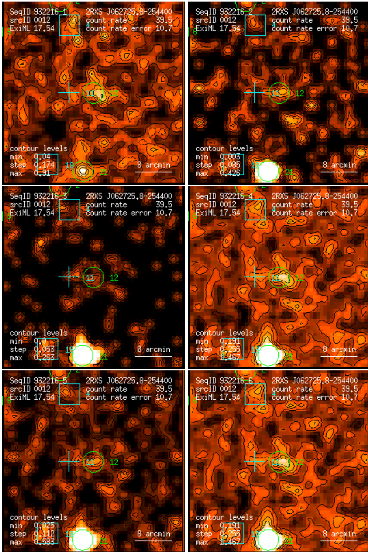
Figure 12: RASS 932216: detection 0012: band rate images, Gaussian filter: (1) PSPC channels 11 – 41, (2) 52 – 90, (3) 91 – 201, (4) 11 – 235, (5) 52 – 201, (6) 11 – 201. Broad band rates in counts/ks. Band rate contour levels in counts/ks/arcmin 2 .
