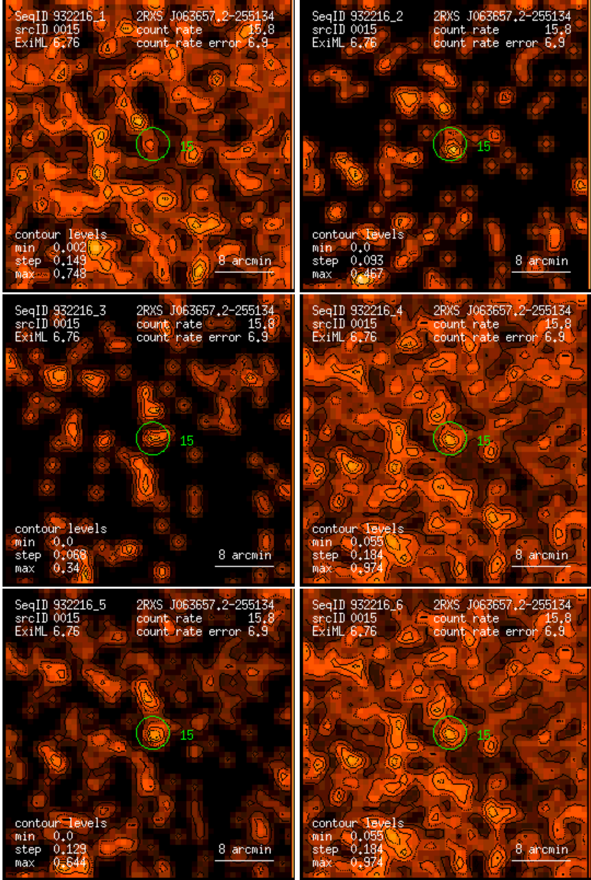
Figure 15: RASS 932216: detection 0015: band rate images, Gaussian filter: (1) PSPC channels 11 – 41, (2) 52 – 90, (3) 91 – 201, (4) 11 – 235, (5) 52 – 201, (6) 11 – 201. Broad band rates in counts/ks. Band rate contour levels in counts/ks/arcmin 2 .
