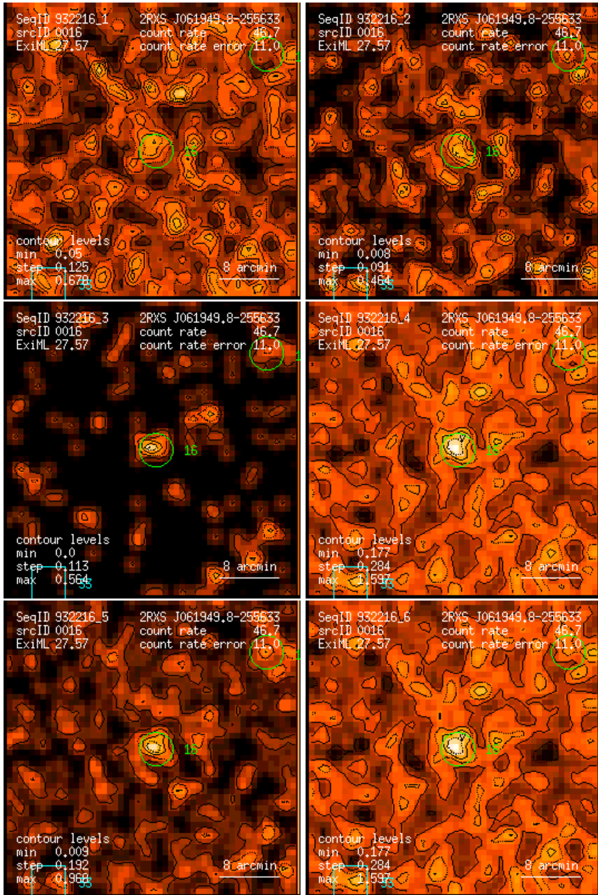
Figure 16: RASS 932216: detection 0016: band rate images, Gaussian filter: (1) PSPC channels 11 – 41, (2) 52 – 90, (3) 91 – 201, (4) 11 – 235, (5) 52 – 201, (6) 11 – 201. Broad band rates in counts/ks. Band rate contour levels in counts/ks/arcmin 2 .
