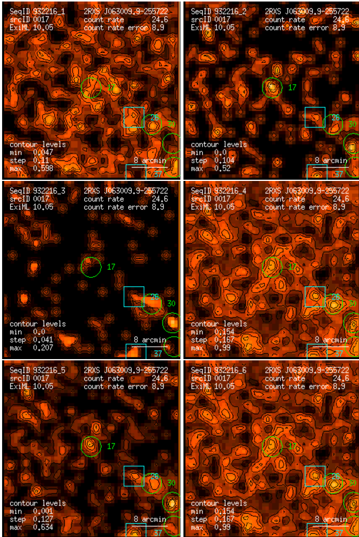
Figure 17: RASS 932216: detection 0017: band rate images, Gaussian filter: (1) PSPC channels 11 – 41, (2) 52 – 90, (3) 91 – 201, (4) 11 – 235, (5) 52 – 201, (6) 11 – 201. Broad band rates in counts/ks. Band rate contour levels in counts/ks/arcmin 2 .
