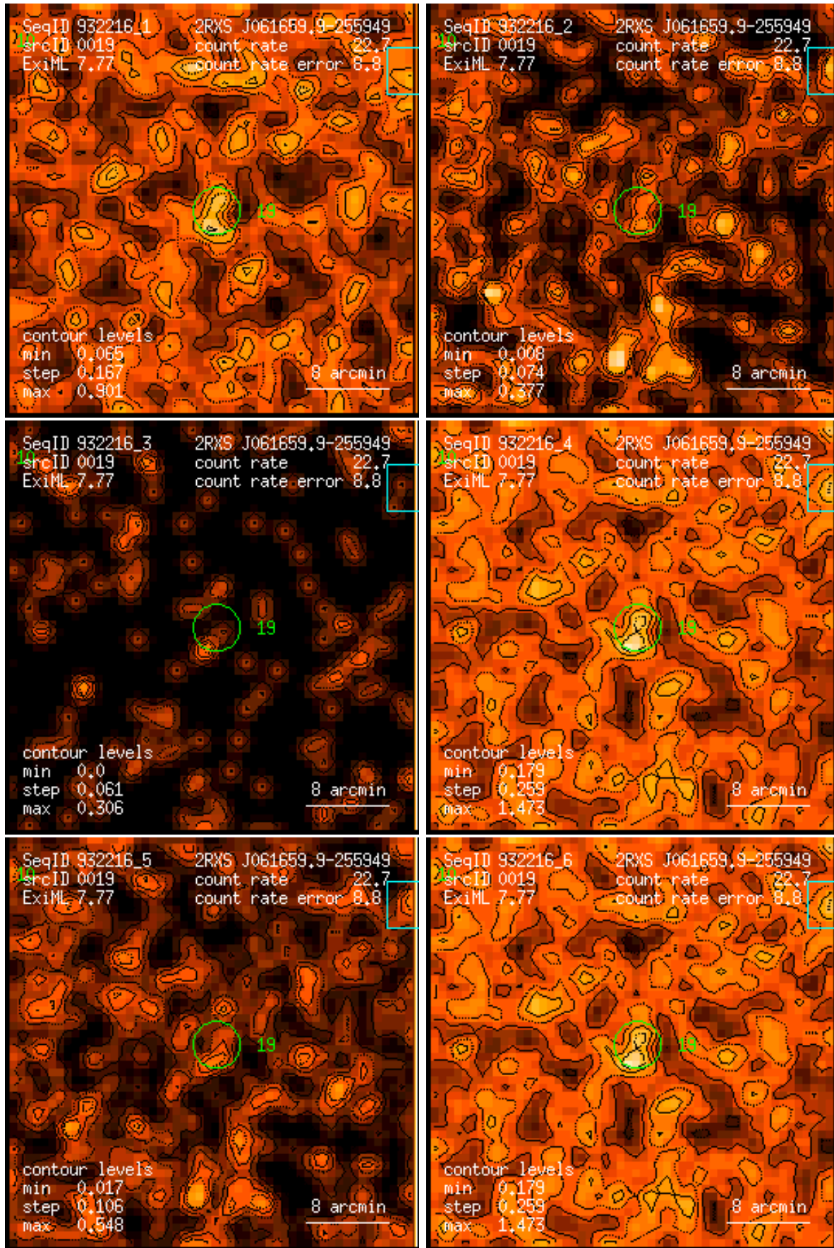
Figure 19: RASS 932216: detection 0019: band rate images, Gaussian filter: (1) PSPC channels 11 – 41, (2) 52 – 90, (3) 91 – 201, (4) 11 – 235, (5) 52 – 201, (6) 11 – 201. Broad band rates in counts/ks. Band rate contour levels in counts/ks/arcmin 2 .
