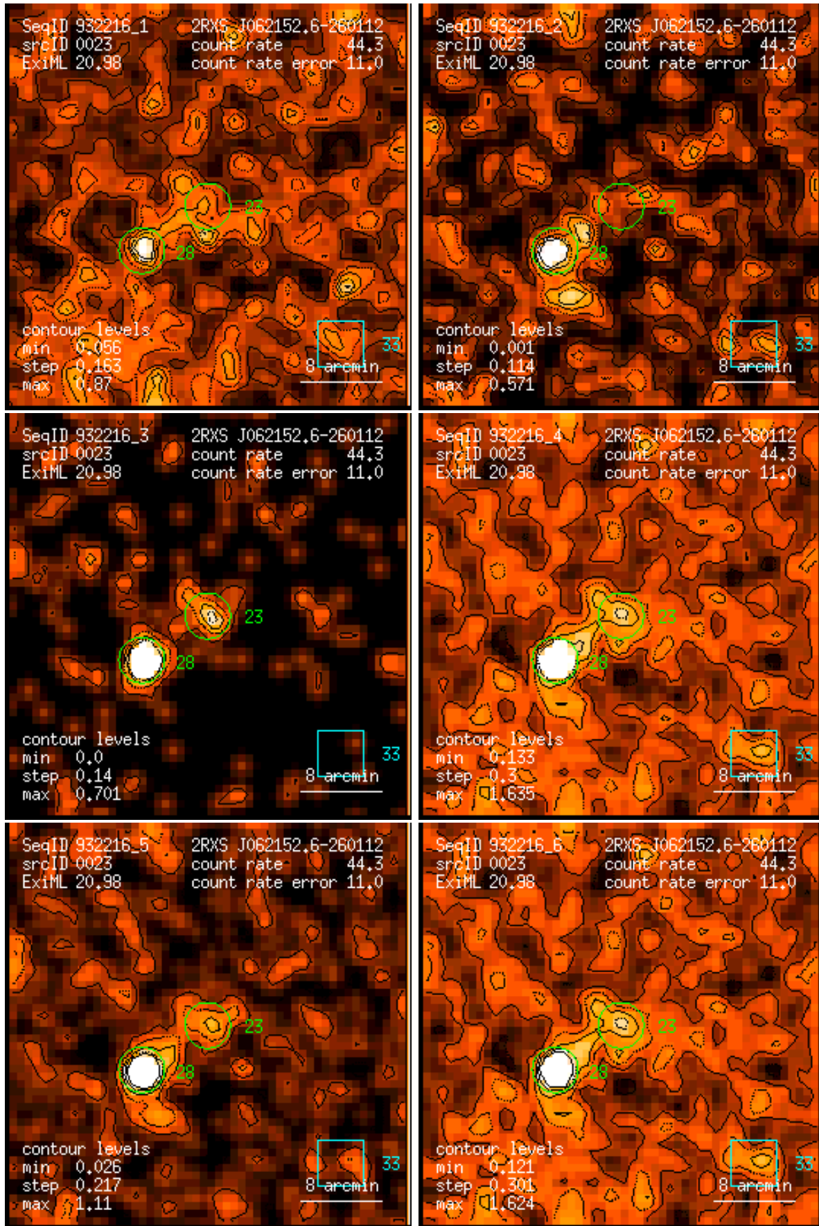
Figure 23: RASS 932216: detection 0023: band rate images, Gaussian filter: (1) PSPC channels 11 – 41, (2) 52 – 90, (3) 91 – 201, (4) 11 – 235, (5) 52 – 201, (6) 11 – 201. Broad band rates in counts/ks. Band rate contour levels in counts/ks/arcmin 2 .
