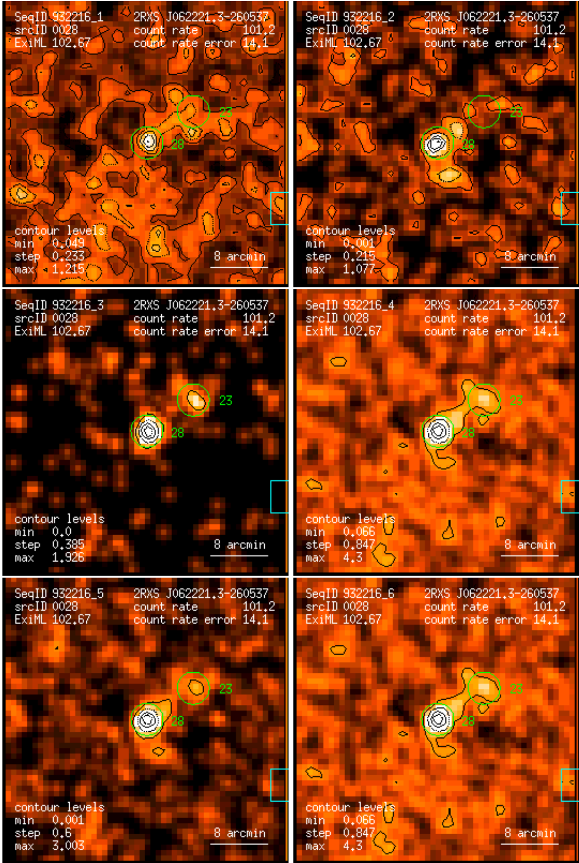
Figure 28: RASS 932216: detection 0028: band rate images, Gaussian filter: (1) PSPC channels 11 – 41, (2) 52 – 90, (3) 91 – 201, (4) 11 – 235, (5) 52 – 201, (6) 11 – 201. Broad band rates in counts/ks. Band rate contour levels in counts/ks/arcmin 2 .
